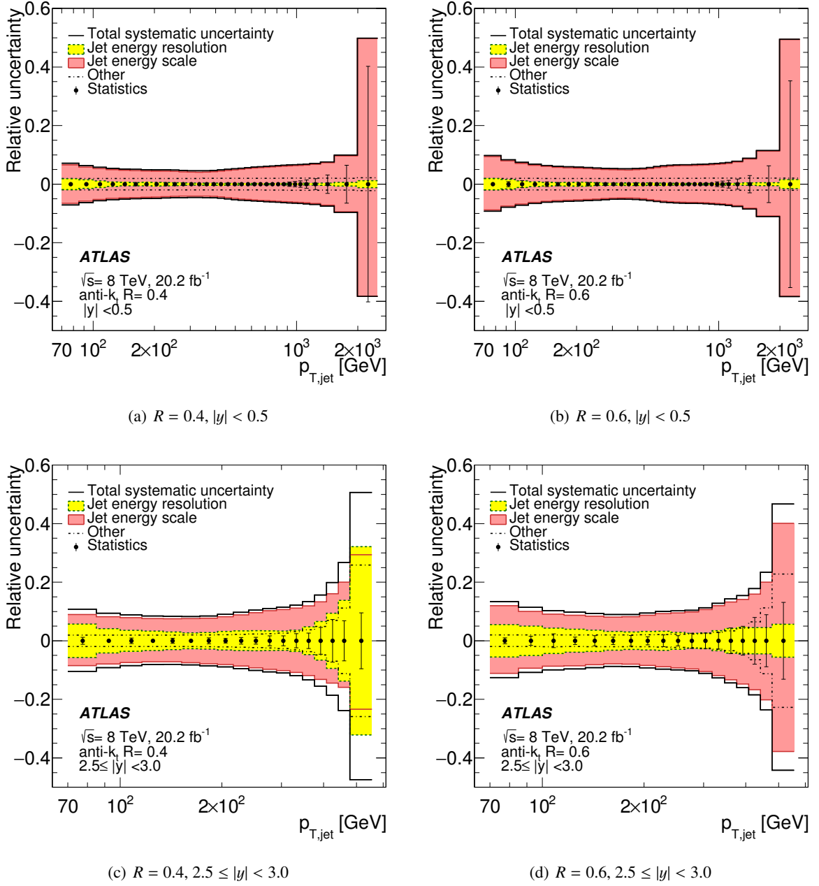
Figure 1: Relative systematic uncertainty for the inclusive jet cross-section as a function of the jet transverse momentum p_{T,jet} . The total systematic uncertainty is shown by the black line. The individual uncertainties are shown in colours: the jet energy scale (red), jet energy resolution (yellow) and the other uncertainties (JAR, jet selection, luminosity and unfolding bias) added in quadrature. The results are shown for the (a,b) first and (c,d) last jet rapidity bins and for anti- k_r jets with (a,c) R = 0.4 and (b,d) R = 0.6 . The statistical uncertainty is shown by the vertical error bar on each point.
