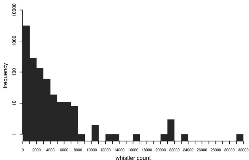
Figure 3. Histogram showing the frequency of daily whistler counts (number of whistlers/day) in AKST/AKDT time from years 2005 to 2013. Each bin width is 1000 whistler counts. On the local day of Mount Okmok’s eruption, the whistler count reached over 21,000 whistlers. Only 0.3% of all days in the data set had a whistler count higher than 8000 counts.
