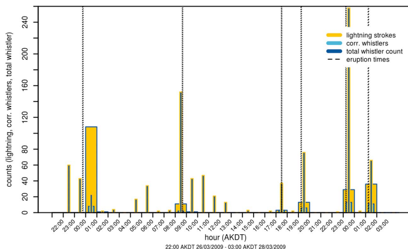
Figure 5. Hourly lightning events and whistler correlation counts for Mount Redoubt from 22.00 AKDT, 26 March 2009 to 3.00 AKDT, 28 March 2009 (yellow and light blue bars) and hourly total whistler counts at Dunedin during the same time frame (dark blue bars). Eruptions on these days were reported to have occurred at 22:48 (26 March), 8:39, 17:35, 19:20, 23:20 (27 March), and 1:20 (28 March) AKDT.
