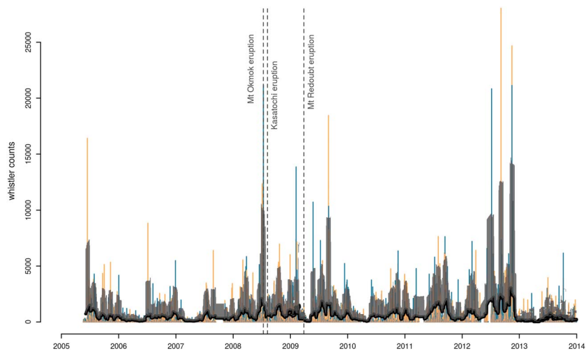
Figure 2. Twenty-four hour whistler counts from year 2005 to 2013 (binned by AKST/AKDT time). Blue and yellow bars represent whistler counts on odd and even days. The black line with gray bands show the rolling mean with a window of 31 days and an uncertainty band of 2\sigma . The day of Mount Okmok’s eruption is the third highest peak in this time period (However, if binned by UTC time, this day drops down to the sixth highest peak). The eruption dates of the three active Aleutian Island volcanoes are marked by dashed lines.
