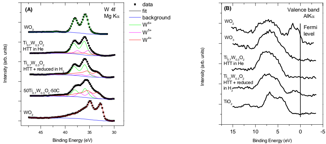
Fig. 4 (A): W 4f core level spectra of the non-reduced and the reduced carbon-free Ti_{0.7}W_{0.3}O_2 samples (route II), and the reduced 50Ti_{0.7}W_{0.3}O_2-50C composite (route III) along with reference spectra of WO_3 and WO_2 . (B): valence band spectra of the non-reduced and the reduced carbon-free Ti_{0.7}W_{0.3}O_2 samples compared with the spectra of WO_2 , WO_3 and TiO_2 .
