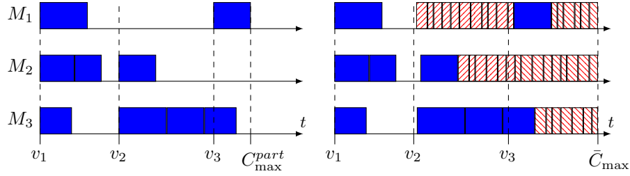
Figure 2: A partial schedule on the left and the schedule was created by Algorithm C2 after \ell = 2 on the right.
