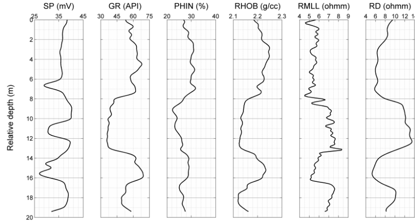
Figure 5. The well logs measured in Well-1 as input for the GA-based interval inversion procedure. Denotations: spontaneous potential (SP), natural \gamma -ray intensity (GR), density (RHOB), neutron porosity (PHIN), microlaterolog (RMLL), deep resistivity (RD).
