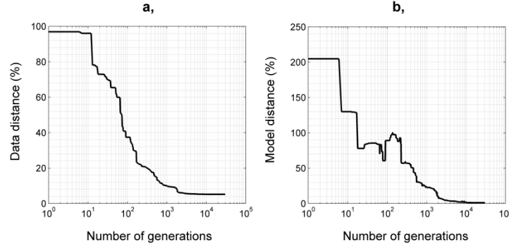
Figure 4. The convergence plots of the GA-based interval inversion procedure: a, data distance of the best individual vs. iteration step, b, model distance of the best individual vs. iteration step.
