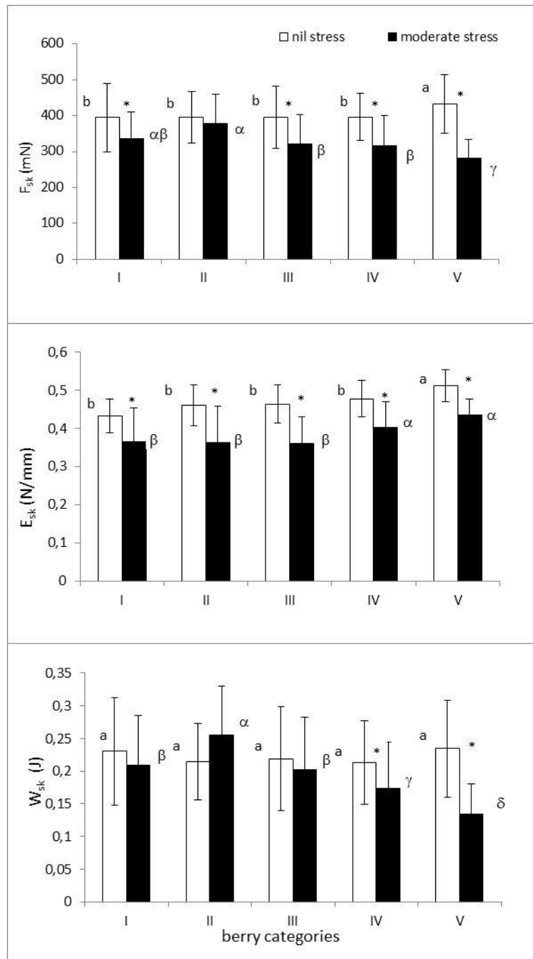
Fig. 6. Results of puncture test conducted on the berries according to berry weights. F_{sk} =skin break force, E_{sk} =skin Young's modulus, W_{sk} =skin break energy. Each column represents the average \pm standard error of 25 replicates. Columns marked * are significantly different from each other. Different letters indicate significant differences between the berry weight categories (greek letters – moderate water stress; roman letters – nil stress) according to Tukey's test ( P < 0.05 ).
