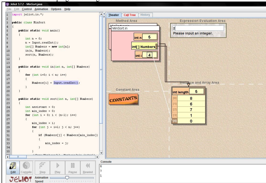
Figure 1. Jeliot
