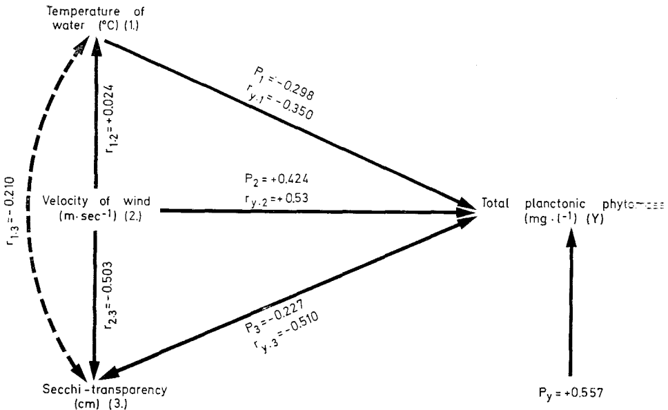
Fig. 10. The Path diagram
