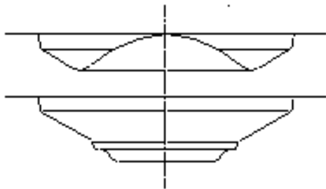
Fig. 3. Modified technologically feasible process plan applying reverse drawing
