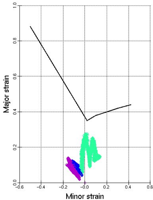
Fig. 6. Forming limit diagram for the 2nd technological variant
