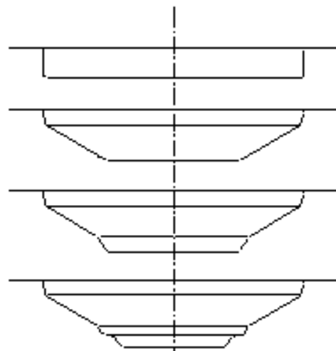
Fig.2. Geometric process plan generated by the Expert System called DEEPEX
