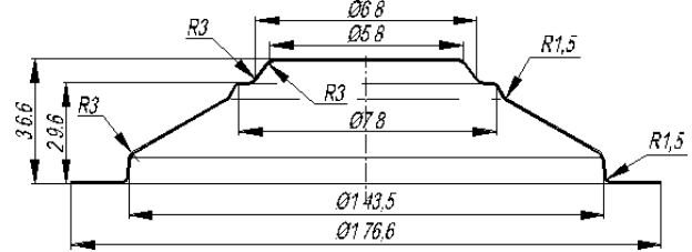
Fig. 1. Geometry of the component to be produced with multi-step sheet forming
