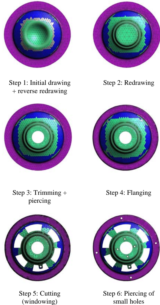
Fig. 7. Simulation results of the 2 nd technological variant including all operations
