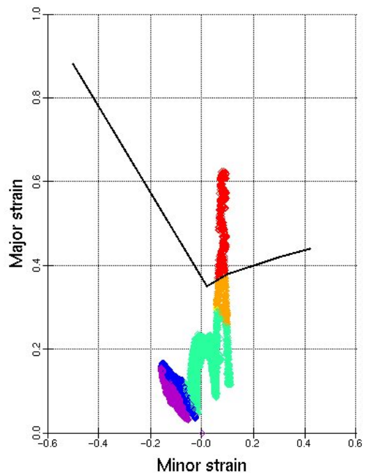
Fig. 5. Forming limit diagram for the 1 st technological variant after the 3 rd drawing step
