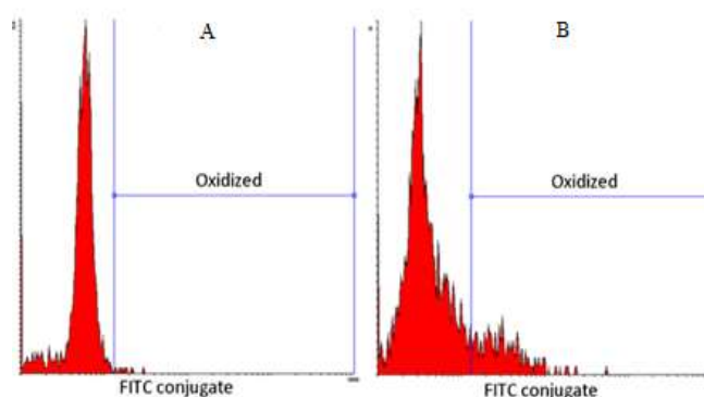
Figure 4. Oxidative DNA lesions in spermatozoa after 30 minutes exposure in the control (A) and in the influent sewage sample (B)
