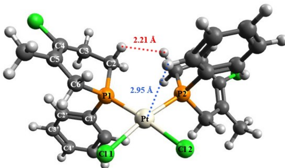
FIGURE 4 Perspective view of cis - bis (4-chloro-1-phenyl-5-methyl-1,2,3,6-tetrahydrophosphinino)-dichloro-platinum(II) [( R,R )- 3 ] calculated by the \omega B97X-D/cc-pVTZ//RI-B97-D/6-31G(d) method. For Pt atoms, cc-pVTZ-PP pseudopotential was applied in all cases. Grey, white grey, orange, green and white colours are referred to carbon, hydrogen, phosphorus, chlorine and platinum atoms, respectively. Selected bond lengths (Å), bond angles (°) and torsion angles (°) are as follows: Pt-Cl(1) 2.394, Pt-P(1) 2.252, P(1)-C2 1.858, C2-C3 1.542, C3-C4 1.515, C4-C5 1.351, C5-C6 1.523, P(1)-C6 1.861, P(1)-C1' 1.832, C1'-C2' 1.411, C2'-C3' 1.403, C3'-C4' 1.404; Cl(1)-Pt-Cl(2) 88.7, Cl(1)-Pt-P(1) 83.8, Pt-P(1)-C2 121.7, Pt-P(1)-C6 110.8, Pt-P(1)-C1' 113.0, P(1)-C2-C3 112.7, C2-C3-C4 114.7, C3-
