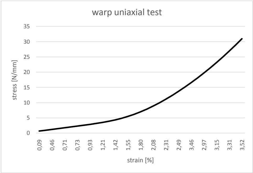
Figure 1. Measured stress, a typical stress-strain curve of a uniaxial tensile test in the warp direction.
