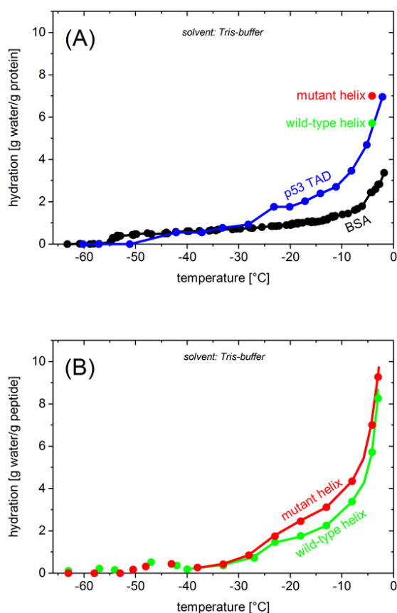
Fig. 2. Hydration measured by the ^1\text{H-NMR} signal intensities of the mobile water for (A) 50 mg/ml p53 TAD (blue circles) and 50 mg/ml BSA (black circles) dissolved in Tris-buffer. The T = -4^\circ\text{C} data for the helix peptides (green and red circles) are the same as in graph (B). (B) 30 mg/ml wild type p53 TAD helix peptide (green circles) and 30 mg/ml mutant helix peptide (red circles) dissolved in Tris-buffer; alternately, the hydration given in units of mole mobile water per mole peptide. Tris-buffer: 150 mM NaCl, 50 mM Tris, 1 mM EDTA, pH 7.5. The lines are guides to the eye.
