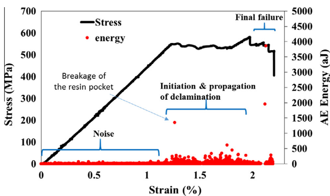
Fig. 9. Stress–strain and AE event energy for pure delamination in a typical [G_4/C_8/G_4] with a pre-cut in the TR30 carbon layer. (For interpretation of the references to colour in this figure legend, the reader is referred to the web version of this article.)
