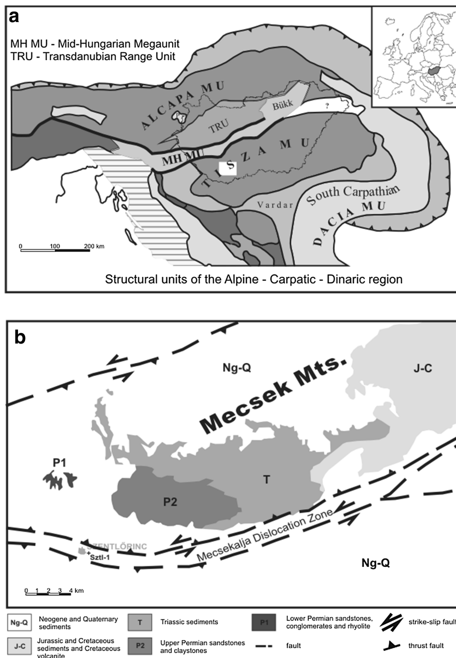
Fig. 1 a Location of the study area (white square) inside of the Pannonian Basin (based on Haas et al. 2010). b The Mecsekajla Zone with the studied Szentlőrinc-1 (Sztl-1) well (based on Konrád et al. 2010)
