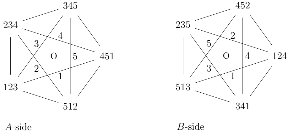
Figure 1: Any three of the 2-bodies, A_i \cup B_i , 0 \leq i \leq 5 , intersect, and they do not have a (1 - 1) -transversal
