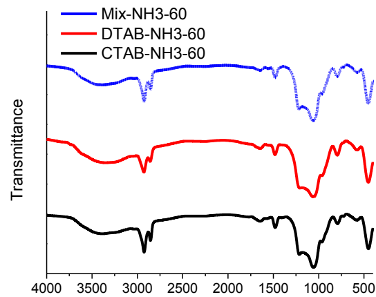
Figure 3. FT-IR spectra of the silica xerogels made with \text{NH}_3 catalyst
