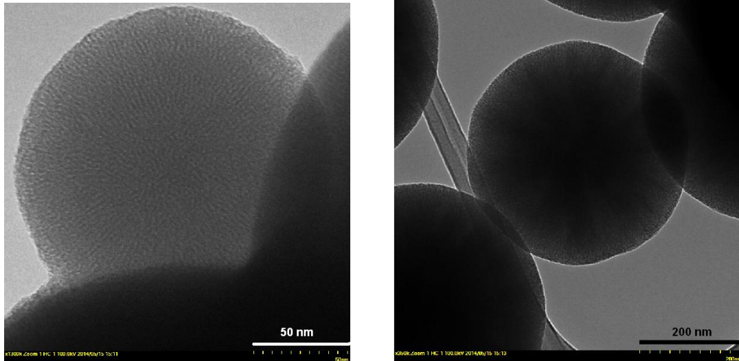
Figure 8. TEM images of silica particles for samples CTAB-NH3-700
