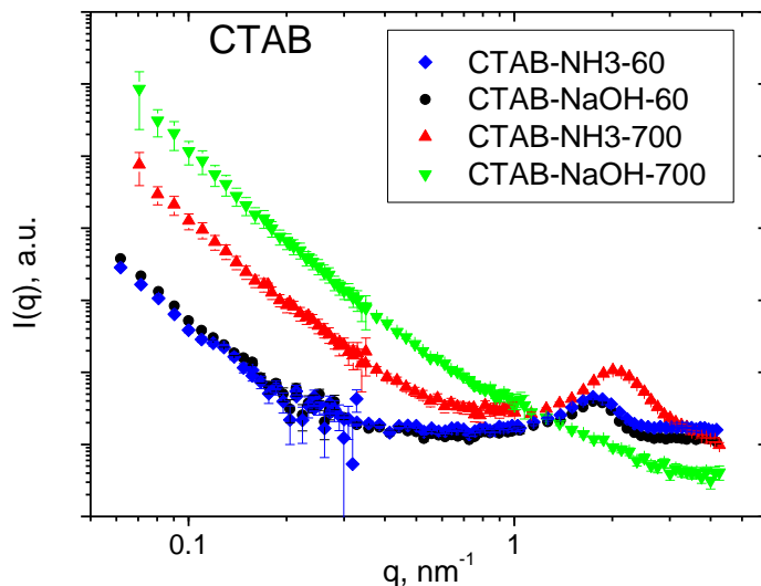
Figure 10 SANS data of samples prepared with CTAB
