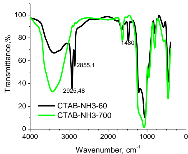
Figure 4. FT-IR spectra of the CTAB-NH3 sample before and after calcination at 700^\circ\text{C}
