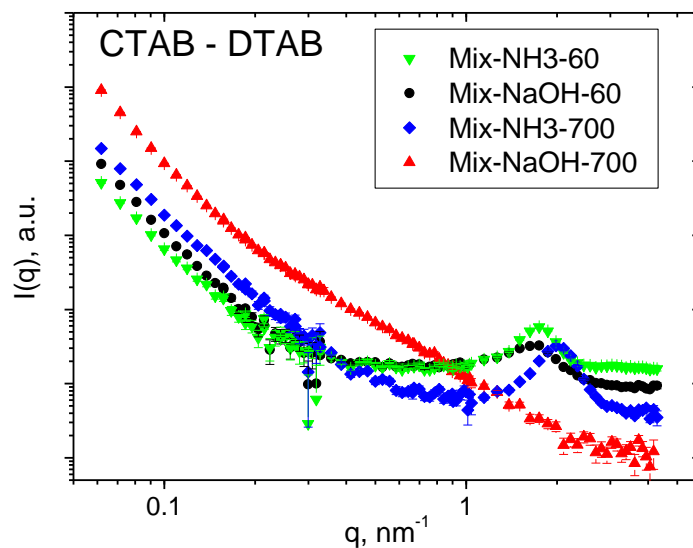
Figure 12. SANS data on samples made with CTAB-DTAB mixed templating agent
