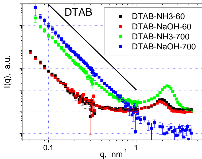
Figure 11. SANS data on samples made with DTAB. The solid line is an asymptote of the power law I(q) \sim q^{-4} .
