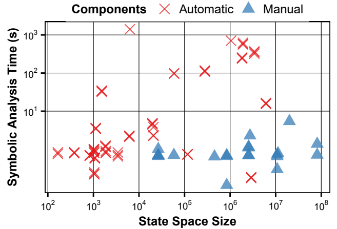
Fig. 6. Execution times of the symbolic part of the analysis.
