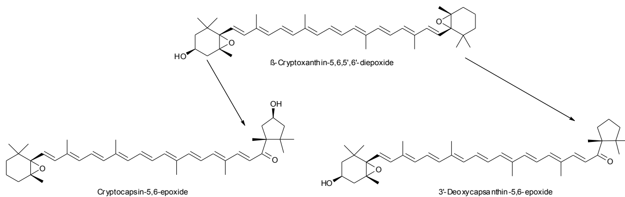
Scheme. 1. Formation of cryptocapsin-5,6-epoxide ( 5 ) and 3'-deoxycapsanthin-5,6-epoxide ( 6 ) from β-cryptoxanthin-5,6,5',6'-diepoxide ( 8 )
