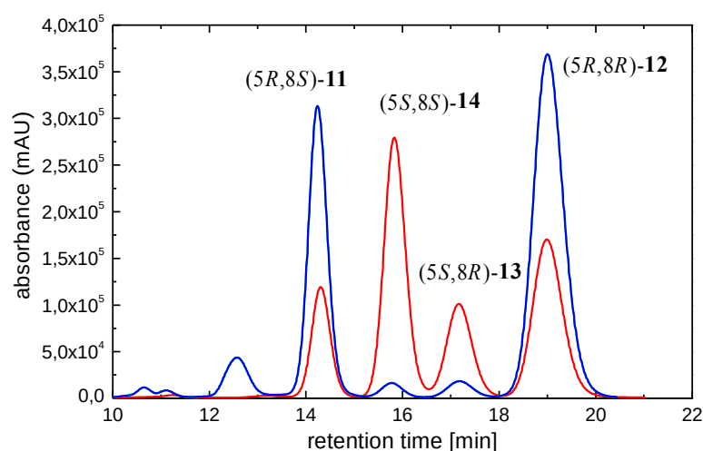
Figure 4. Overlapped HPLC-UV traces (463 nm) of natural [blue, ( 5R,8S,3'S,5'R )- 11 , ( 5R,8R,3'S,5'R )- 12 ] and semisynthetic stereoisomeric mixture of cryptocapsin-5,8-epoxides [red, ( 5R,8S,3'S,5'R )- 11 , ( 5R,8R,3'S,5'R )- 12 , ( 5S,8R,3'S,5'R )- 13 , ( 5S,8S,3'S,5'R )- 14 ] with Chiralpak IC column ( n -hexane/EtOH 80:20);
