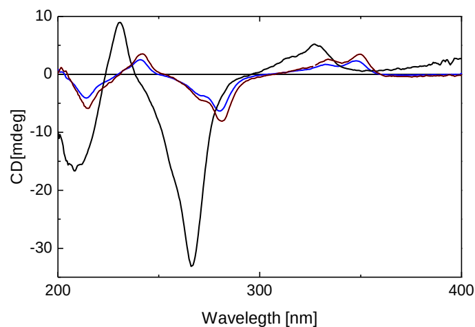
Figure 1. ECD spectra of (5 R ,6 S ,3' S ,5' R )-cryptocapsin-5,6-epoxide ( 5 , red) (3 R ,5 R ,6 S ,5' R )-3'-deoxycapsanthin-5,6-epoxide ( 6 , blue) and (3 S ,5 R ,6 S ,5' R ,6' S )- \beta -cryptoxanthin-5,6,5',6'-diepoxide ( 8 , black).
