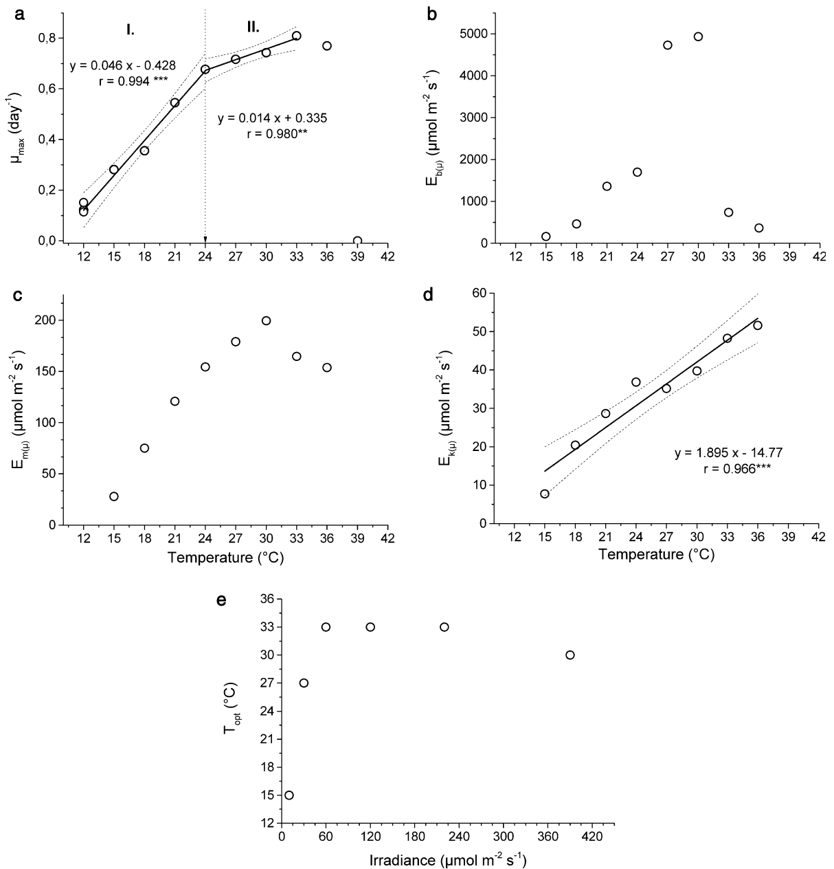
Fig. 3 Estimated physiological parameters for growth–irradiance relationship of Cylindrospermopsis raciborskii (ACT 9502) at different temperatures used by Platt et al. (1980) model; a \mu_{\text{max}} , the maximum growth rate at optimal irradiance at a particular temperature; as a consequence of the impossibility of fitting at 12 °C, each \mu'_{\text{max}} value of the triplicate was
