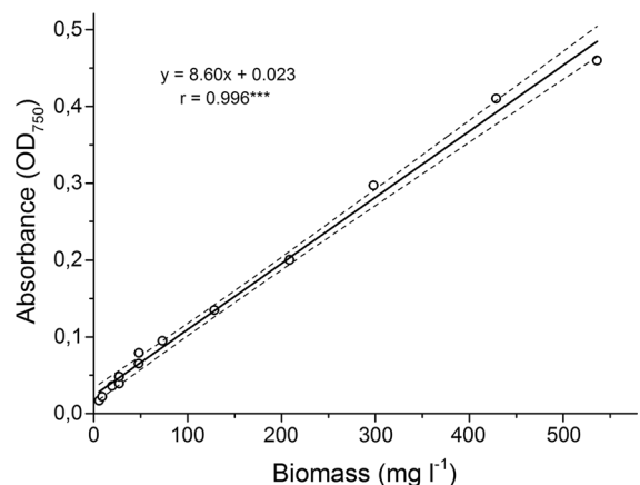
Fig. 1 Correlation between the absorbance measured at 750 nm ( \text{OD}_{750} ) and the biomass of filaments of Cylindrospermopsis raciborskii (ACT 9502). The solid line is the regression through the data, and dashed lines are the 95 % confidence intervals
