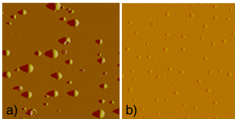
Figure 5 AFM images of surface blisters. (a) Sample hydrogenated at 1.5 ml/min and annealed for 1 h (scan size 40 \mu\text{m} ) and (b) sample hydrogenated at 0.4 ml/min and annealed for 4 h (scan size 10 \mu\text{m} ).
