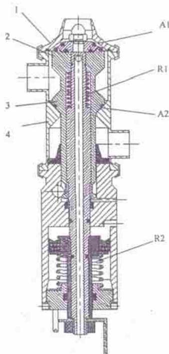
Figure 1. The cutaway view of valve
