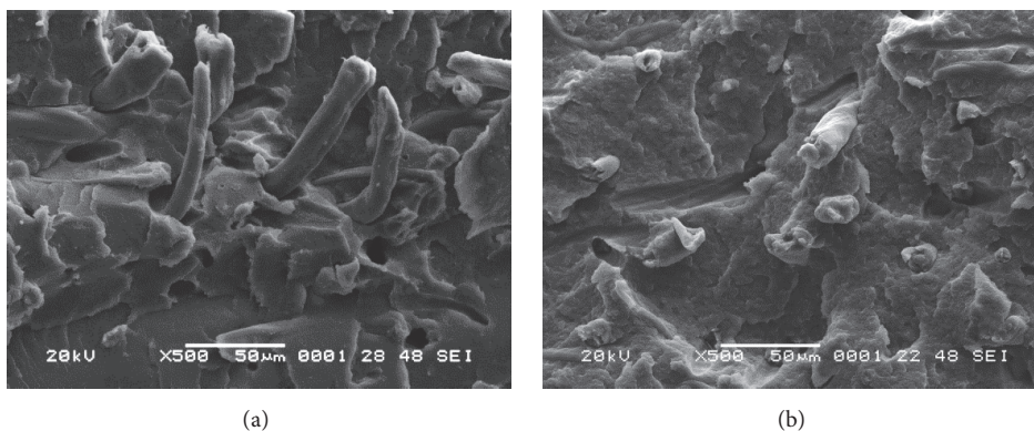
FIGURE 11: Fracture surface micrographs for 90/10 w/w PLA/HENCEL composites: (a) without and (b) with PLA-g-MA coupling agent.
