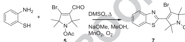
Scheme 2. Reaction of compound 5 with 2-aminothiophenol in dimethyl sulfoxide (DMSO) in the absence of base.
