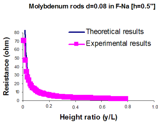
FIG. 16 COMPARISON BETWEEN EXPERIMENTAL RESULTS AND ANALYTICAL RESULTS OBTAINED FROM CIRCUIT MODEL NORMALIZED FOR MOLYBDENUM RODS OF DIAMETER D=0.08 INCH AND RODS' SEPARATION DISTANCE H=0.5 INCH F-NA.
