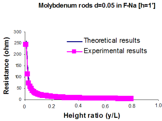
FIG. 15 COMPARISON BETWEEN EXPERIMENTAL RESULTS AND ANALYTICAL RESULTS OBTAINED FROM CIRCUIT MODEL NORMALIZED FOR MOLYBDENUM RODS OF DIAMETER D=0.05 INCH AND RODS' SEPARATION DISTANCE H=1 INCH IN F-NA.
