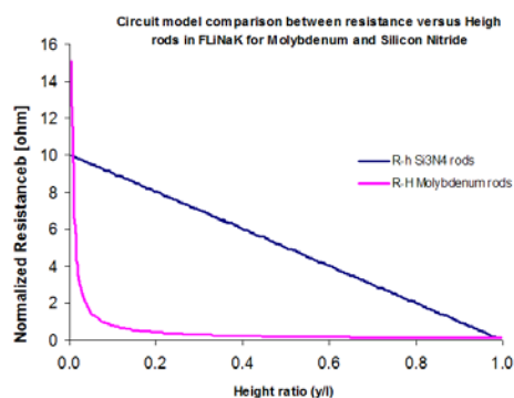
FIGURE 25 : COMPARISON OF ANALYTICAL SOLUTION OF RODS OF DIFFERENT MATERIAL ( \text{Si}_3\text{N}_4 , MOLYBDENUM) IN THE SAME LIQUID SOLUTION (FLiNaK)
