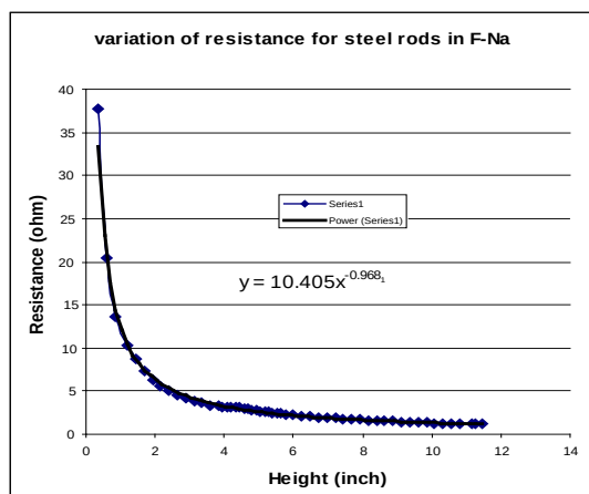
FIG 3 RESISTANCE BETWEEN STEEL RODS IN F-NA WATER SOLUTION VERSUS LIQUID LEVEL
