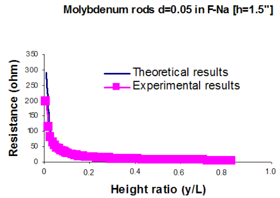
FIG. 18 COMPARISON BETWEEN EXPERIMENTAL RESULTS AND ANALYTICAL RESULTS OBTAINED FROM CIRCUIT MODEL NORMALIZED FOR MOLYBDENUM RODS OF DIAMETER D=0.05 INCH AND RODS' SEPARATION DISTANCE H=1.5 INCH F-NA.
