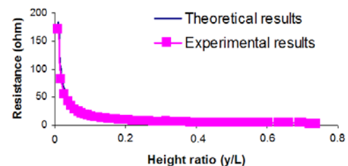
FIG. 13 COMPARISON BETWEEN EXPERIMENTAL RESULTS AND ANALYTICAL RESULTS OBTAINED FROM CIRCUIT MODEL NORMALIZED FOR MOLYBDENUM RODS OF DIAMETER D=0.05 INCH AND ROD SEPARATION DISTANCE H=0.5 INCH NAF.
