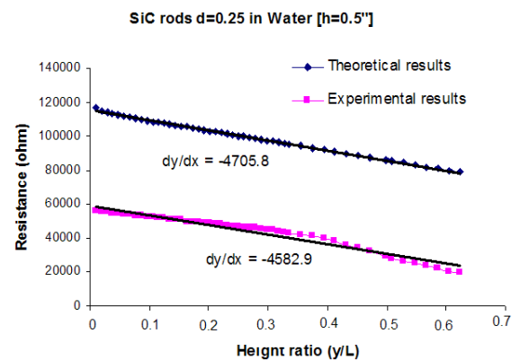
FIG. 20 COMPARISON BETWEEN EXPERIMENTAL RESULTS AND ANALYTICAL RESULTS OBTAINED FROM CIRCUIT MODEL FOR SiC RODS OF DIAMETER D=0.25 INCH AND RODS' SEPARATION DISTANCE H=0.5 INCH WATER.
