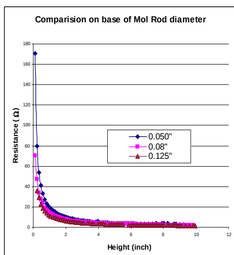
FIG. 7 COMPARISON OF RESISTANCE VERSUS HEIGHT OF MOLYBDENUM RODS WITH DIFFERENT DIAMETER SUBMERGED IN THE NaF SOLUTION
