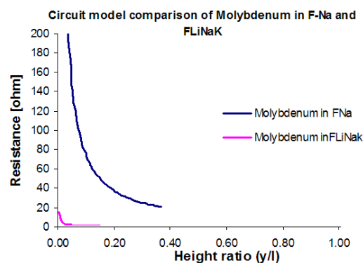
FIGURE 24: CAPARISON OF ANALYTICAL SOLUTION OF MOLYBDENUM RODS IN DIFFERENT LIQUID SOLUTION (NAF IN WATER, FLINAK)
