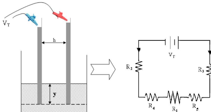
FIG. 12 CORRESPONDING ELEMENTS IN CIRCUIT MODEL FOR THE RESISTANCE BASE HIGH TEMPERATURE LIQUID LEVEL SENSOR
