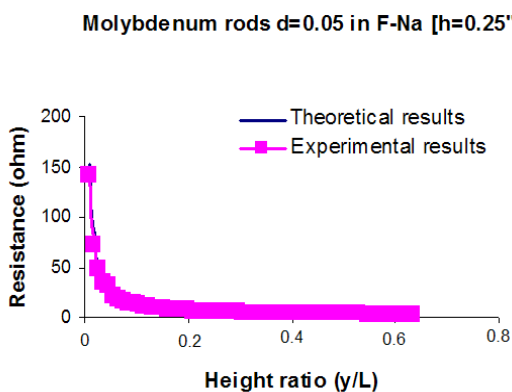
FIG. 17 COMPARISON BETWEEN EXPERIMENTAL RESULTS AND ANALYTICAL RESULTS OBTAINED FROM CIRCUIT MODEL NORMALIZED FOR MOLYBDENUM RODS OF DIAMETER D=0.05 INCH AND RODS' SEPARATION DISTANCE H=0.25 INCH F-NA.
