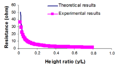
FIG. 14 COMPARISON BETWEEN EXPERIMENTAL RESULTS AND ANALYTICAL RESULTS OBTAINED FROM CIRCUIT MODEL NORMALIZED FOR MOLYBDENUM RODS OF DIAMETER D=0.125 INCH AND RODS' SEPARATION DISTANCE H=0.5 INCH NAF.
