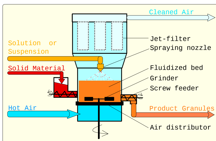
Fig. 1. Fluidized bed drier and granulator
