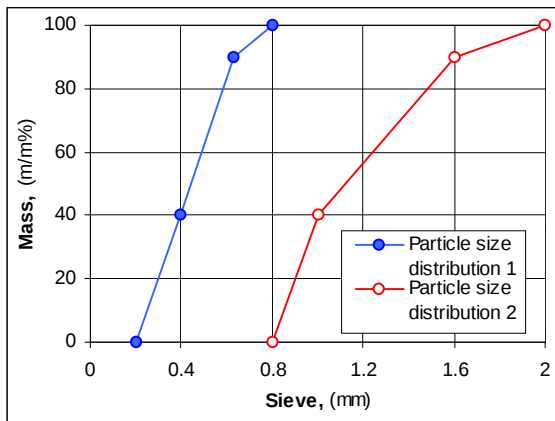
Figure 8: Particle size distributions for powders in experiment depicted in Figure 9.
