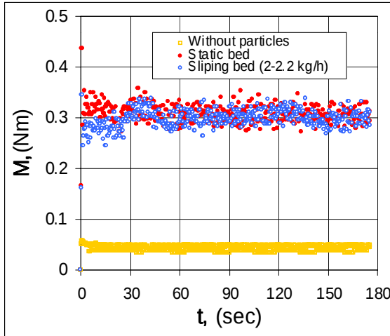
Fig. 6. Torque vs. time in static and slipping beds
