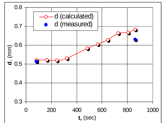
Figure 9: Average particle size from torque and direct measurements.
