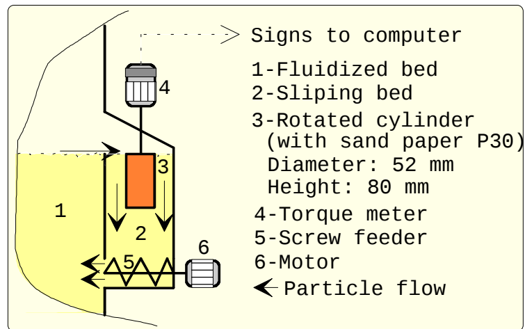
Fig. 3. Modified Couette-device connected to the fluidized bed granulator
