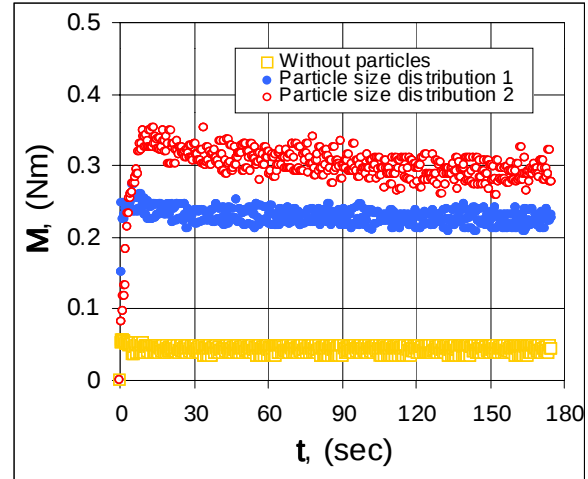
Fig. 7. Torque vs. time at different particle size distributions
