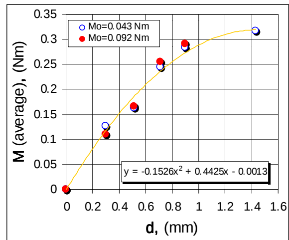
Fig. 5. Mean particle size vs. average torque
