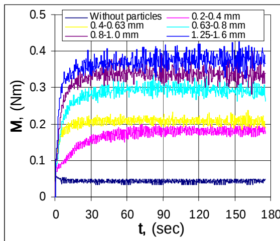
Fig. 4. Torque vs. time
