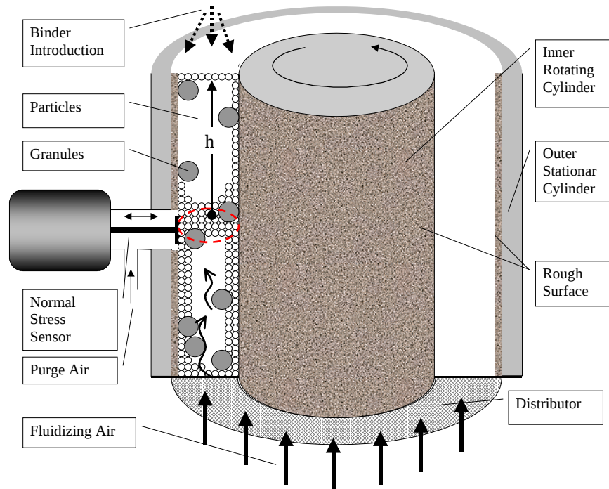
Fig. 2. Schematic diagram of the Cuette-device used by Tardos et al. [2]
