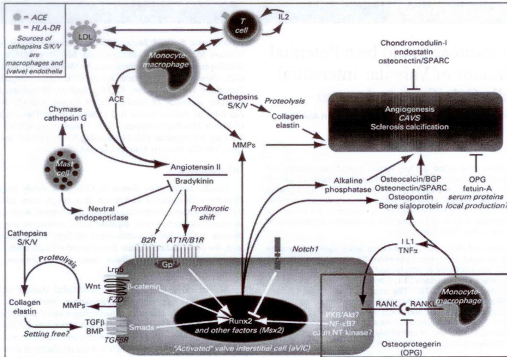
Figure 1: Convergence of regulatory pathways in the activation of VICs. The red rectangle highlights the action of RANKL and the natural inhibition by OPG [2].
