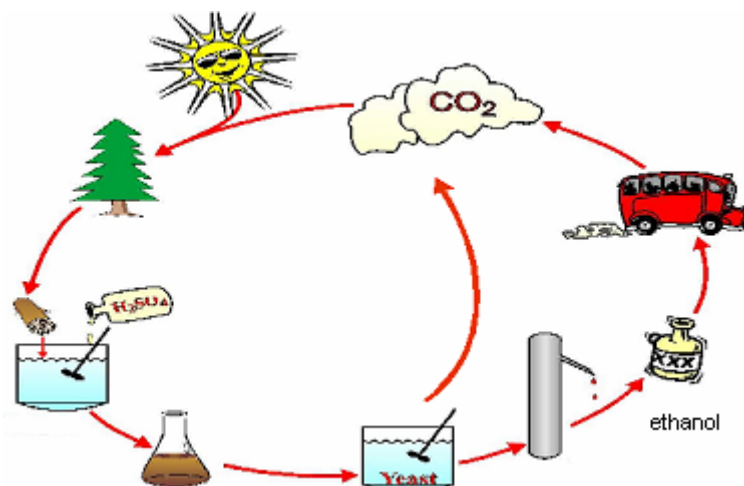
Fig. 1. The closed CO 2 cycle of the biologically produced ethanol (5)
