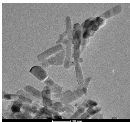
Figure 1. TEM image of titania nanorods ( \text{TiO}_2 NR)
