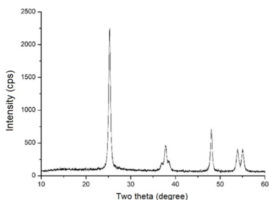
Figure 2. XRD of titania nanorods ( \text{TiO}_2 NR)
