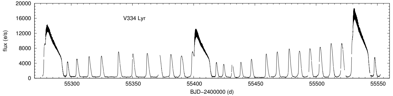
Figure 4. Light curve of V334 Lyr, an SU UMa-type dwarf nova from Kepler quarters 5, 6, and 7, spanning 276 days. Notice the normal and superoutbursts throughout observations. In the case of all superoutbursts a trigger (normal) outburst can be seen.
