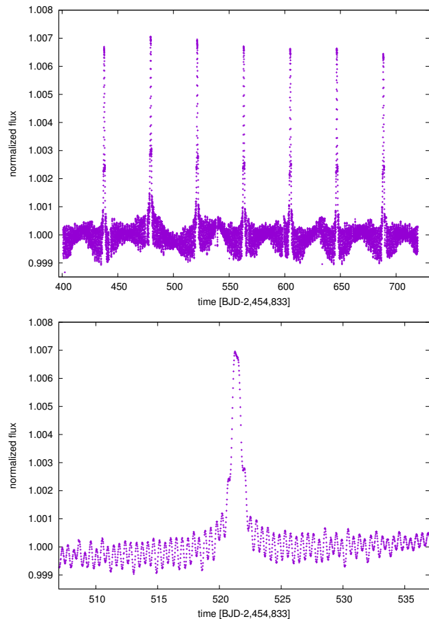
Figure 6. Top: The Kepler light curve of KOI-54, a heart-beat star. Bottom: A zoom-in in the light curve of KOI-54. In between the brightenings the system shows tidally induced oscillations.
