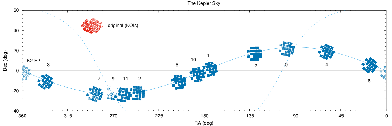
Figure 1. The observing fields of Kepler in the sky. For the original field (red) we only plotted the KOIs ( Kepler Object of Interest) instead of all targets. K2 fields include the positions of all observed targets and pixel mosaics. In Campaign 9 most of the pixels were assigned to a smaller, but continuous area to search for microlensing events, hence the sparse coverage for the other CCD modules.
