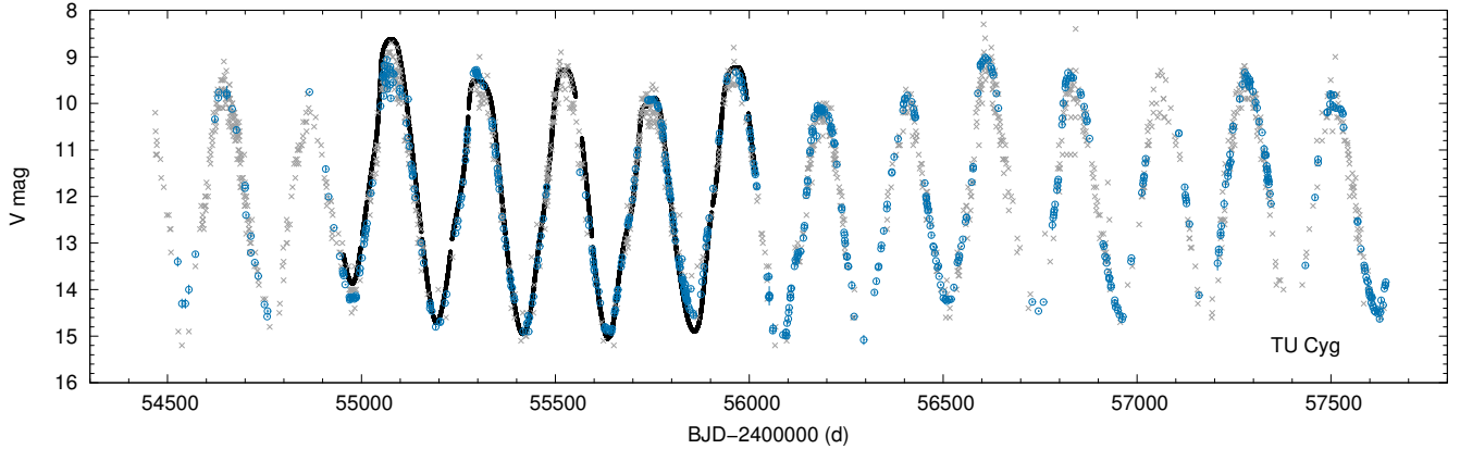
Figure 2. A comparison of the AAVSO visual (grey), digital V -band and green-filter (blue) observations and the Kepler light curve (black) of the Mira star TU Cyg. Here we used the data from between 01/01/2009 and 16/09/2016. The corrected Kepler data, published by Bányai et al. (2013) , have is scaled to the amateur observations.
