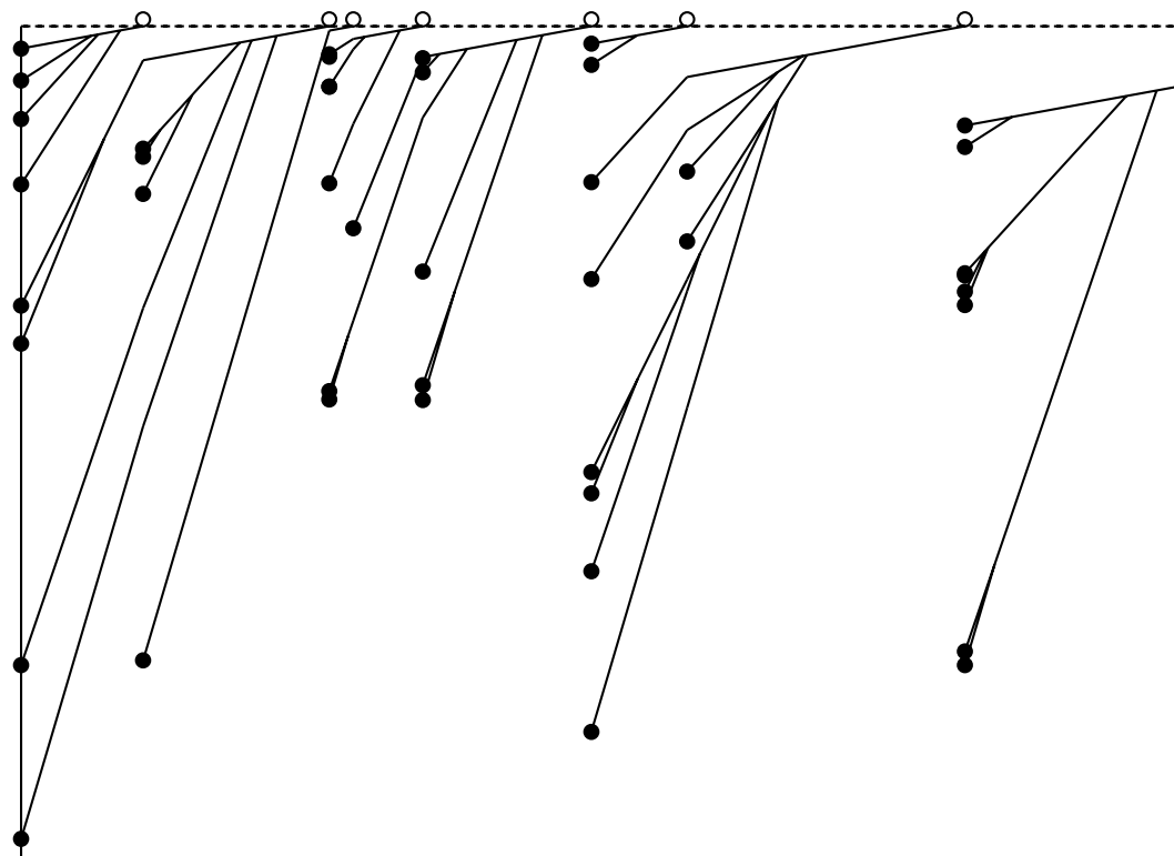
Figure 6: A simulation of the particle system realising the forest fire model. The system has n = 8 particles and \lambda = 0.4 , and is shown on the time interval [0, 2] . Compare to the systems realising the MCLD and the multiplicative coalescent in Figures 2 and 3. The burning events (which occur when a block reaches 0) here involve blocks of sizes 4, 7, 1, 5, 8, 2, 8 respectively. Note that in this case the process of burnings is a Poisson process of rate n\lambda .
