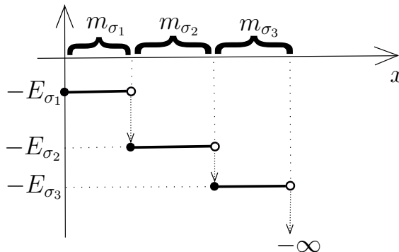
Figure 4: An illustration of the function f_0 defined in (2.7) when n = 3 .
