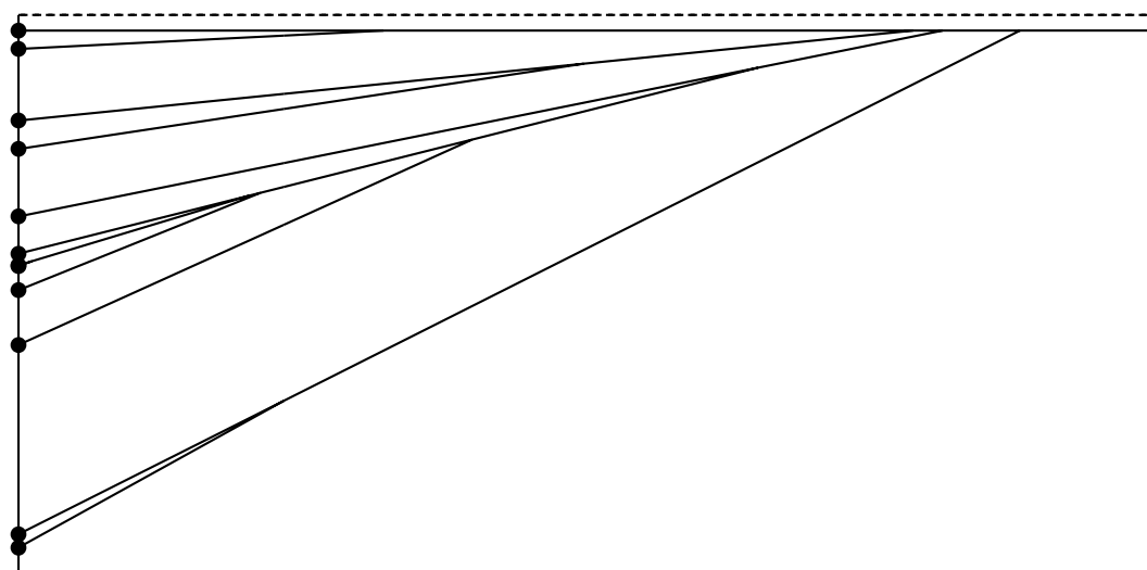
Figure 3: This shows a similar system to the one in Figure 2, but now with \lambda = 0 so that the system realises the multiplicative coalescent, with no deletion. In this case n = 12 and the figure shows the time interval [0, 0.25] . By the end, all particles have coalesced into a single block.
