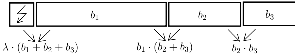
Figure 1: An illustration of the rates of the interval coalescent process: the lengths of the three intervals (from left to right) are b_1 , b_2 and b_3 . The leftmost block marked with a lightning represents the “cemetery”. The rate at which the first interval gets deleted is \lambda \cdot (b_1 + b_2 + b_3) . The rate at which the first interval merges with the second one is b_1 \cdot (b_2 + b_3) . The rate at which the second and third intervals merge is b_2 \cdot b_3 .
