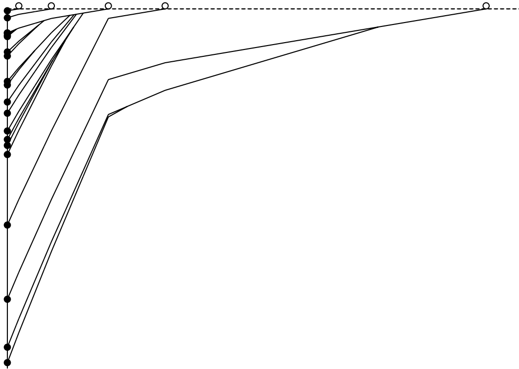
Figure 2: A simulation of the particle system which realises the MCLD. Each particle moves upwards at rate equal to \lambda plus the mass of particles strictly above it. When a particle reaches 0 it dies and is removed from the system. Particles at the same height at time t form a time- t block. The figure shows a system with n = 20 particles and \lambda = 1.3 , evolving on the time interval [0, 0.5] . We see 5 deletion events, and the deleted blocks have sizes 1, 1, 14, 1, 3 respectively. Compare to Figure 3, where \lambda = 0 (realising the multiplicative coalescent without deletion), and to Figure 6, where deleted particles reenter at independent exponential heights (realising the forest fire model).
