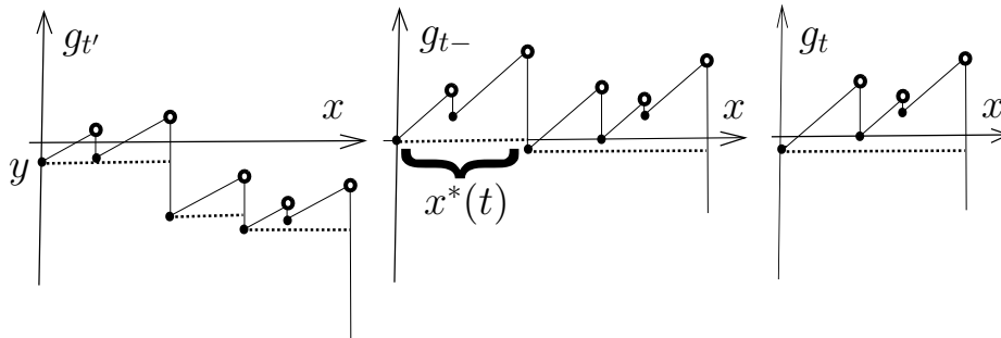
Figure 5: An illustration of Definition 2.9. Dashed lines are used to denote the running minimum. The second graph g_{t-} is obtained from the first graph g_{t'} using the tilt operation. Observe that some excursions of g_{t'} got merged with the tilt operation. The third graph g_t is obtained from the second graph by shifting it to the left by x^*(t) , i.e., the length of the first excursion of the second graph. If we denote by y the level of the first excursion of g_{t'} then t = t' + |y|/\lambda is the time instant when this excursion reaches level zero and thus gets shifted.
