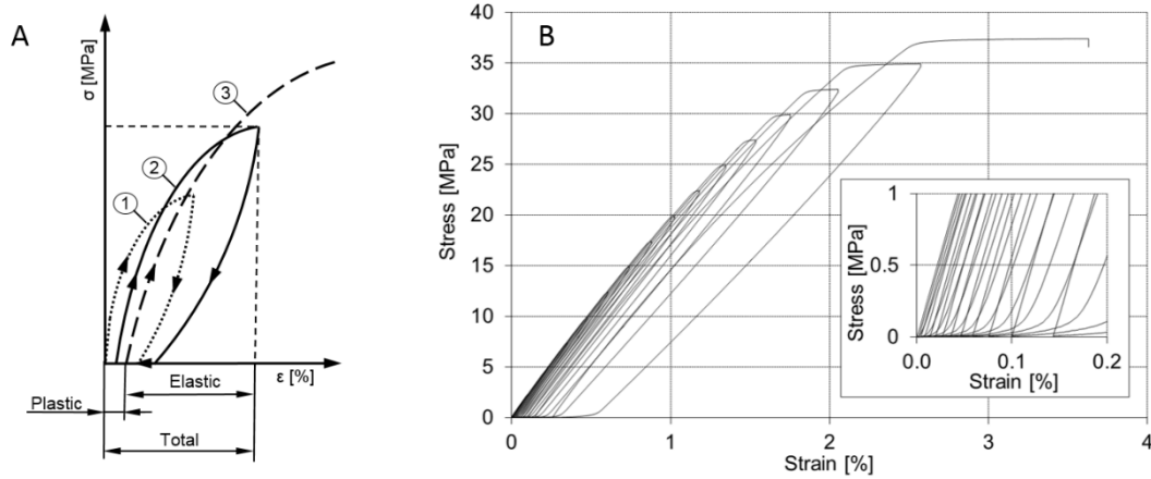
Figure 2. Strain-stress curves for cyclic loading, at increasing load levels A shows an idealized curve (the solid curve (2) is a complete cycle) and B shows a real measurement curve in the case of PA 6+MMT
