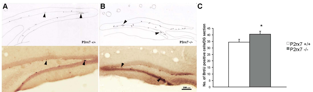
Figure 5. Summary of BrdU staining in P2rx7+/+ (A) and P2rx7-/- (B) mice. A, B/Representative sections show rostral hippocampal DG areas in 1 \times 1 sections of male wild type and P2rx7 knock out mice. Dark dots (arrowheads) represent the BrdU-positive cells (ImmPress-DAB-Ni staining). Camera lucida drawings of the same sections where the newly formed BrdU-labeled cells are indicated. The microscopic picture and drawing were taken at the same magnification (20X), and the bar indicates 100 \mu m. Histogram showing the average number of BrdU-positive cells in a rostral hippocampal DG area in the granule cell layer and in the 50- \mu m zone adjacent to its inner edge. C/We observed a significant difference (n = 5, p = 0.046) in the average number of labeled cells in the sections of P2rx7+/+ and P2rx7-/- mice. doi:10.1371/journal.pone.0066547.g005
