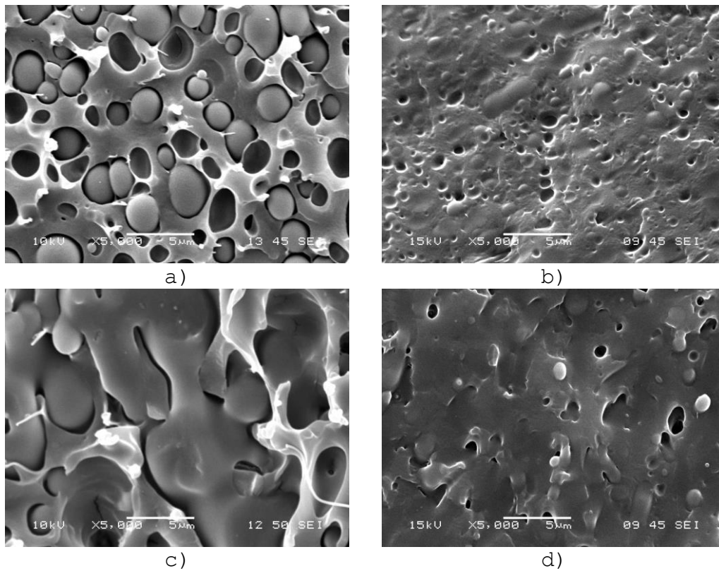
Fig. 5 Morphology of physical (a, c) and reactive (b, d) blends with PLA as matrix containing 0.3 (a, b) and 0.5 volume fraction (c, d) polyurethane elastomer respectively (Magnification: 5000, SEM micrographs taken from cryo-fractured surfaces)
