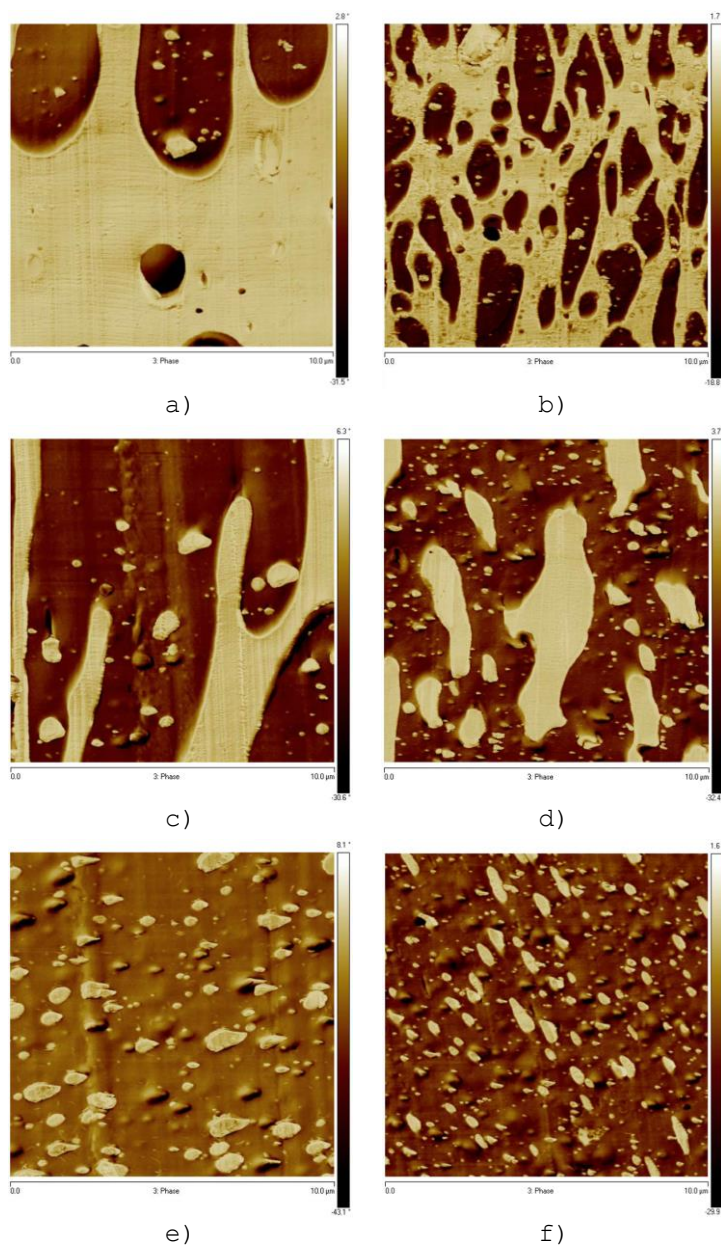
Fig. 6 Morphology of physical (a, c, e) and reactive (b, d, f) blends with PU as matrix containing 0.5 (a, b) 0.3 (c, d) and 0.1 volume fraction (e, f) PLA (tapping mode AFM phase images).
