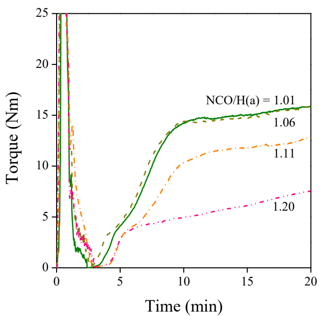
Fig. 2 Changes in torque during reactive blending as a function of time at (a) small and (b) large isocyanate contents with the NCO/H(a) ratio indicated (PLA-b-PU reactive blends containing 0.3 volume fraction PU).
