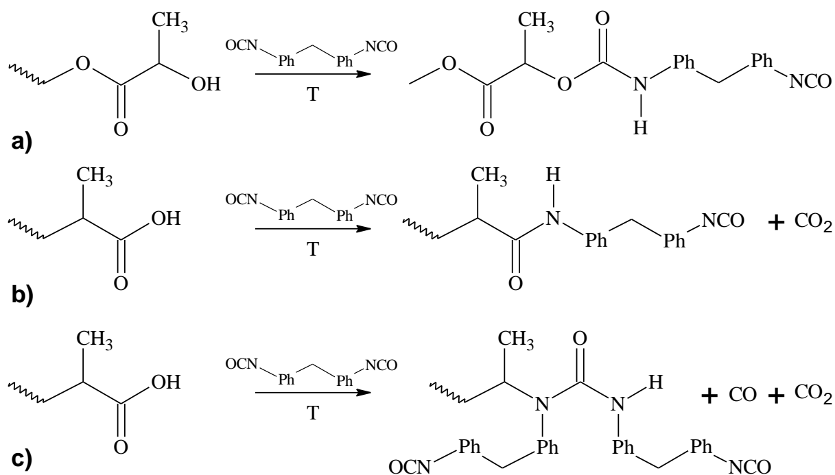
Fig. 1 Hypothetical reactions of MDI with PLA end-groups; a) formation of polyurethane on the hydroxyl end-group, b) formation of amide on the carboxyl end-group, c) formation of acylurea on the carboxyl end-group.
