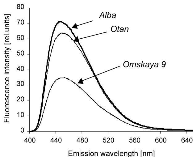
Fig. 1. Emission fluorescence spectra of flag leaf-rolling and non-rolling wheat genotypes. ('Omskaya 9' = non-rolling parents genotyp; 'Otan' = genotype with the most pronounced degree of leaf rolling; 'Alba' = genotype with the middle degree of leaf rolling. All measurements were made on adaxial surface of 8–10 flag leaves per genotype)
