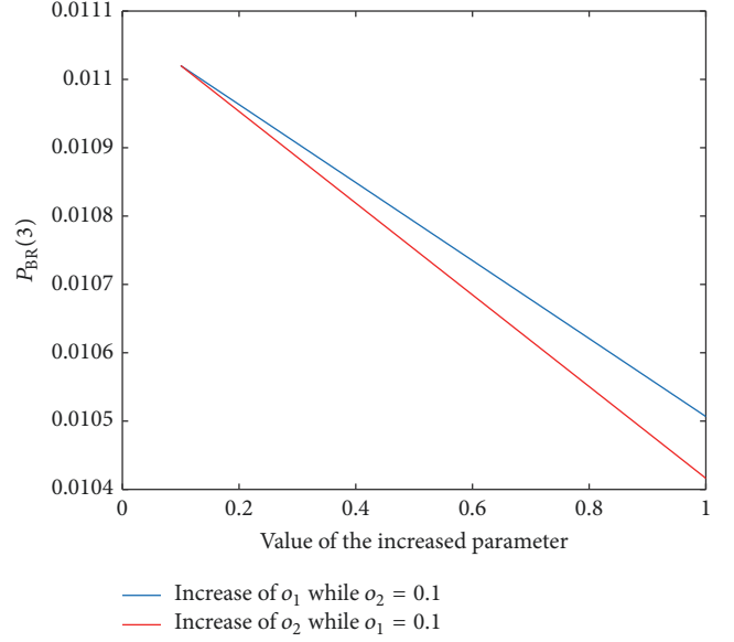
FIGURE 2: P_{BR}(3) as function of the offer. The blue line illustrates the effect when the offer to the degree 1 depositor is increased while the offer to the degree 2 depositor is kept constant at 0.1, while the red line illustrates the dual case.
