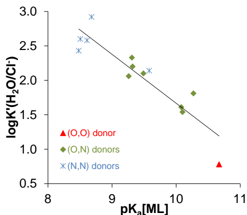
Fig. 6 \log K'(H_2O/Cl^-) values vs. pK_a[ML] for the Rh(\eta^5-C_5Me_5) complexes containing various bidentate ligands with O/N/S donor atoms: R^2 = 0.8403 , \log K'(H_2O/Cl^-) = -0.7095 \times pK_a[ML] + 8.7623 . The coordinated ligands in the complexes used in the correlation are: deferiprone 16 as (O,O) donor, 2-picolinic acid 16 , 6-methylpicolinic acid 17 , quinoline-2-carboxylic acid 17 , 3-isoquinolinecarboxylic acid 17 , 8-hydroxyquinoline 18 , 8-hydroxyquinoline-5-sulfonate 18 and 7-(1-piperidinylmethyl)-8-hydroxyquinoline 18 as (O,N) donors, en 20 , dmen, pin, bpy 20 and phen as (N,N) donors. (See the constants collected in Table S2.)
