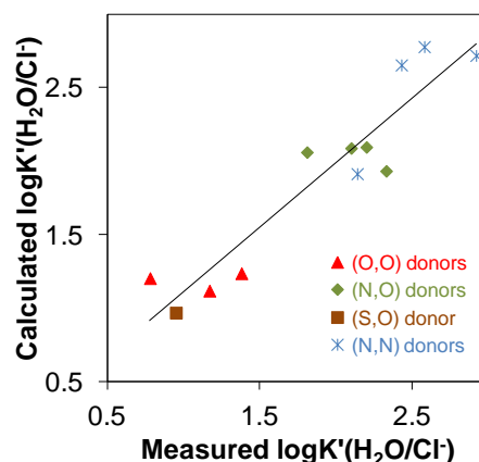
Fig. 7 Multilinear regression between \log K'(H_2O/Cl^-) vs. geometrical parameters: R^2 = 0.8799 ; y = 27.59 \times \text{distance}(\text{Rh-centroid}) - 0.23 \times \text{angle}(X-Rh-X) - 0.23 \times \text{torsion angle}(\text{methyl group-ring plane}) - 28.75 . The coordinated ligands in the complexes used in the correlation are: deferiprone 16 , maltol 15,35 and allomaltol 15 as (O,O) donors, 2-picolinic acid 16,35 , 6-methylpicolinic acid 17 , quinoline-2-carboxylic acid 17 , 8-hydroxyquinoline 18 as (O,N) donors, thiomaltol 19 as (O,S) donor, en 20 , pin, bpy 20,25 and phen 25 as (N,N) donors.
