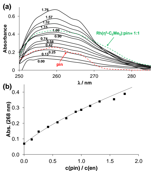
Fig. 5 UV-vis spectra for the displacement study of [\text{Rh}(\eta^5\text{-C}_5\text{Me}_5)(\text{en})(\text{H}_2\text{O})]^{2+} – pin (1:1) system (black solid lines). The numbers show the different c(\text{pin}) -to- c(\text{en}) ratios. The spectra of [\text{Rh}(\eta^5\text{-C}_5\text{Me}_5)(\text{pin})(\text{H}_2\text{O})]^{2+} and pin are shown with dashed lines (a). Absorbance values at 268 nm (■) plotted against the c(\text{pin}):c(\text{en}) ratio, dotted line shows the fitted spectral change (b); spectra are background subtracted \{c_{\text{Rh}} = c_{\text{en}} = 100 \mu\text{M}; I = 0.20 \text{ M KNO}_3, \text{pH} = 7.30, T = 25 \text{ }^\circ\text{C}, l = 1 \text{ cm}\} .
