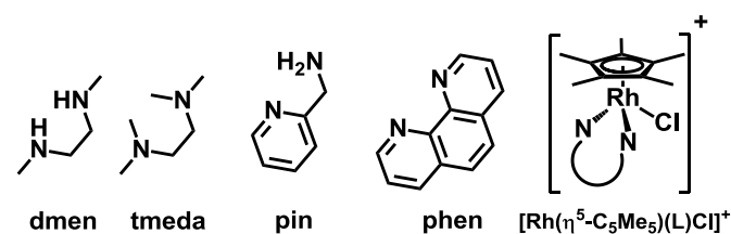
Chart 1 Chemical structures of the ligands: N,N'-dimethylethylenediamine (dmen), N,N,N',N'-tetramethylethylenediamine (tmeda), 2-picolylamine (pin) and 1,10-phenanthroline (phen) and the general formula of the prepared [\text{Rh}(\eta^5\text{-C}_5\text{Me}_5)(\text{L})\text{Cl}]^+ complexes.
