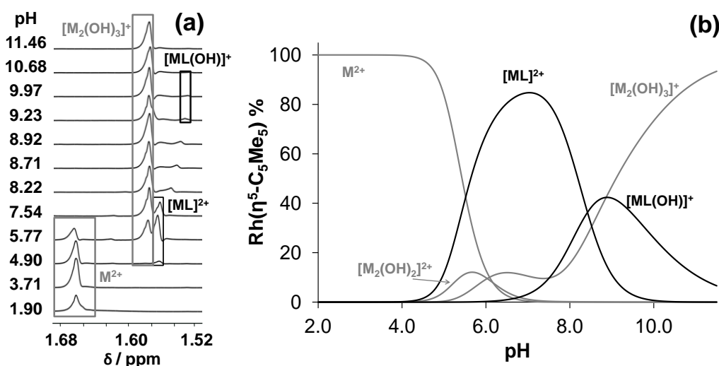
Fig. 4 High-field region of the ^1\text{H} NMR spectra for the [\text{Rh}(\eta^5\text{-C}_5\text{Me}_5)(\text{H}_2\text{O})_3]^{2+} ( \text{M}^{2+} ) – tmeda (1:1) system recorded at the indicated pH values \{C_{\text{Rh}} = C_{\text{tmeda}} = 1 \text{ mM}; T = 25 \text{ }^\circ\text{C}; I = 0.20 \text{ M (KNO}_3\text{)}; 10\% \text{ D}_2\text{O}\} (a). Concentration distribution curves for the [\text{Rh}(\eta^5\text{-C}_5\text{Me}_5)(\text{H}_2\text{O})_3]^{2+} – tmeda (1:1) systems calculated on the basis of the stability constants determined \{C_{\text{Rh}} = C_{\text{tmeda}} = 1 \text{ mM}; T = 25 \text{ }^\circ\text{C}; I = 0.20 \text{ M (KNO}_3\text{)}\} (b).
