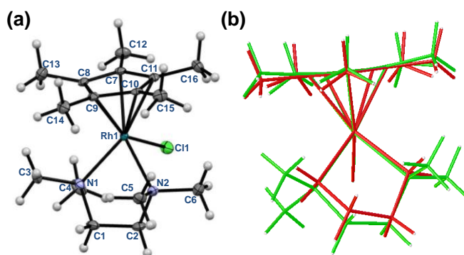
Fig. 2 Molecular structure of 2. Solvent molecules and counter ions are omitted for clarity. Displacement ellipsoids are drawn at 50% probability level (a). Comparison of the molecular structure of complex 2 (coloured with green) with [\text{Rh}(\eta^5\text{-C}_5\text{Me}_5)(\text{en})\text{Cl}]^+ (coloured with red) (b).
