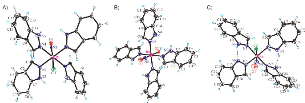
Figure 1. A) ORTEP view of the cation [RuCl(NO)(Hind) 4 ] 2+ in the crystal structure of [ 3 ]Cl 2 ·2(CH 3 ) 2 CO with atom labeling scheme and thermal ellipsoids at 50% probability level; only the major components of the disordered over two positions Cl − and NO are shown. Counterions and solvent molecules in the crystal structure are omitted for clarity. Selected bond distances (Å) and angles (deg): Ru–N1 2.080(6), Ru–N4 2.085(7), Ru–Cl1 i 2.214(7), Ru–N3 1.806(19), N3–O1 1.174(19), Ru–N3–O1 168.9(17), Cl1 i –Ru–N3 174.5(6); B) ORTEP view of the cation [Ru(OH)(NO)(Hind) 4 ] 2+ in the crystal structure of [ 4 ]Cl 2 ·2(CH 3 ) 2 CO with atom labeling scheme and thermal ellipsoids at 50% probability level; only the major components of the disordered over two positions OH − , NO and two indazole ligands are shown. Counterions and solvent molecules in the crystal structure are omitted for clarity. Selected bond distances (Å) and angles (deg): Ru–N1 2.078(3), Ru–N4 2.078(3), Ru–O2 i 1.996(9), Ru–N3 1.702(11), Ru–N3–O1 171.0(9), N3–Ru–O2 i 178.1(6); C) ORTEP view of the neutral complex [RuCl(ind) 2 (Hind) 2 (NO)] [ 5 ] with atom labeling scheme and thermal ellipsoids at 50% probability level. Co-crystallized solvent is omitted for clarity. Selected bond distances (Å) and angles (deg): Ru–N1 2.090(4), Ru–N3 2.094(4), Ru–N5 2.081(4), Ru–N7 2.073(4), Ru–Cl1 2.2959(13), Ru–N9 1.774(5), N9–O1 1.127(6), Ru–N9–O1 168.7(5), N9–Ru–Cl1 174.68(15).
