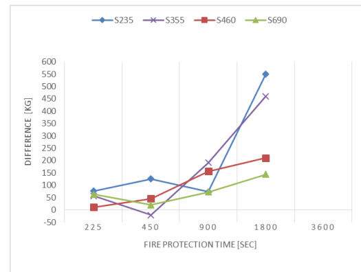
Figure 6. Mass difference between hollow section and welded plate
