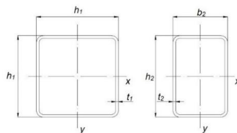
Figure 2. The cross sections of SHS and RHS hollow sections
