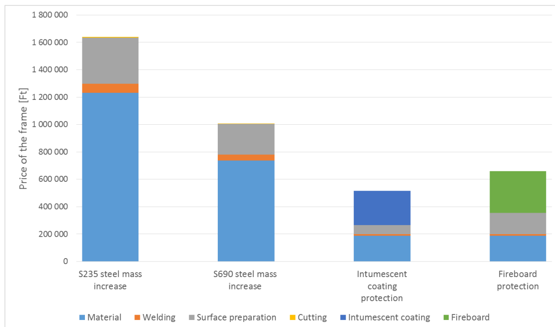
Figure 8. Results of cost calculation (Equal fire protection levels)
