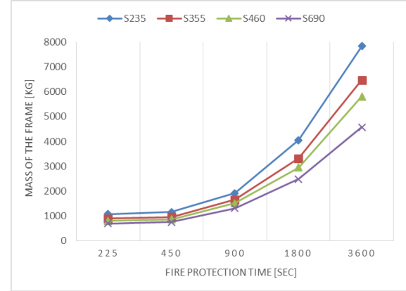
Figure 4. Mass of the frame in case of different types of steel versus fire protection time
