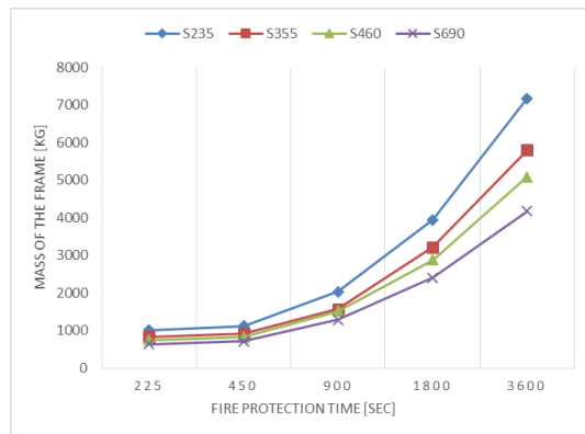
Figure 5. Mass of the frame in case of different types of welded plate versus fire protection time
