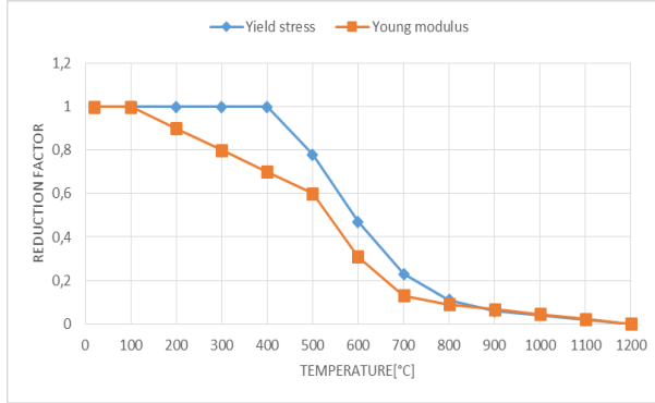
Figure 3. Reduction factor of yield stress and Young modulus versus temperature
