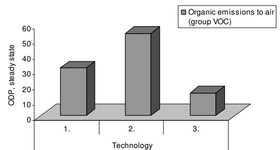
Figure 6: Ozone Layer Depletion Potential (ODP, steady), CML2001
