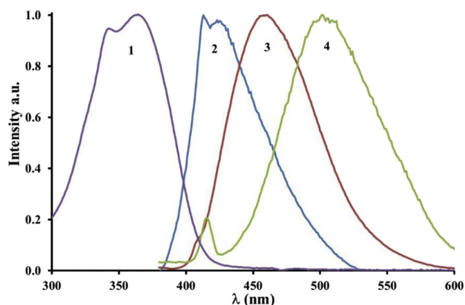
Fig. 1. The normalized absorption (1) and emission spectra of ACAIN recorded in hexane (2), THF (3) and water (4). The absorption spectrum was recorded in THF.
