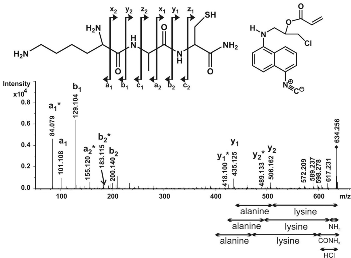
Fig. 5. The tandem mass spectrum of the ACAIN-KAC adduct. The fragment ions marked by asterisks are generated with the loss of \text{NH}_3 from the corresponding product ions. Figure inset shows the structures of the ACAIN and the KAC and the possible generated fragment ions of the KAC molecule.
