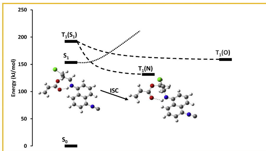
Fig. 7. Electronic energies of the S_1 structure of ACAIN (in hexane) in its S_0 , S_1 and T_1 ( T_1(S_1) ) electronic states. The other two energies correspond to the two triplet minima. The lines are approximations of the S_1 (···) and T_1 (–) potential energy surfaces.
