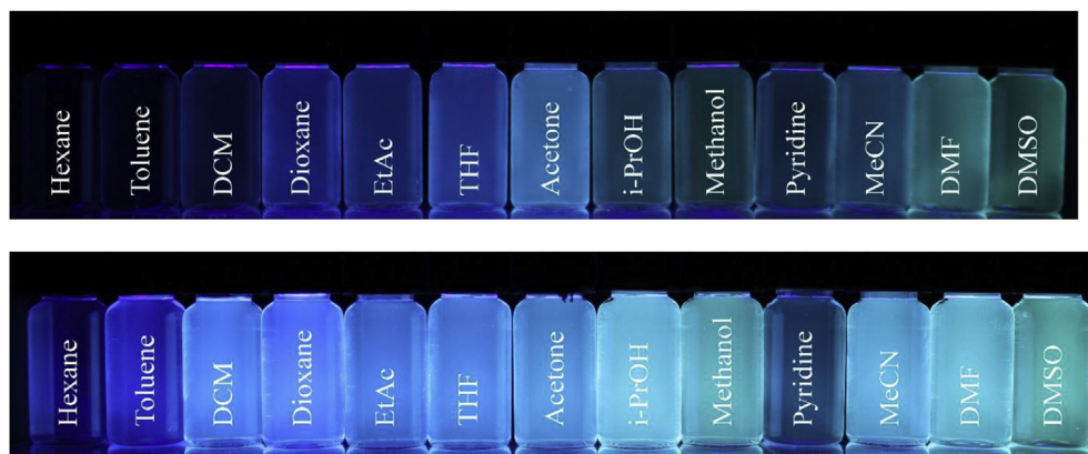
Fig. 3. Visible fluorescence of ACAIN (top) and ACAIN-propanethiol adduct (bottom) in solvents in order of increasing polarity excited at \lambda = 365 nm. All solutions have the same concentration: 25.4 \mu M.
