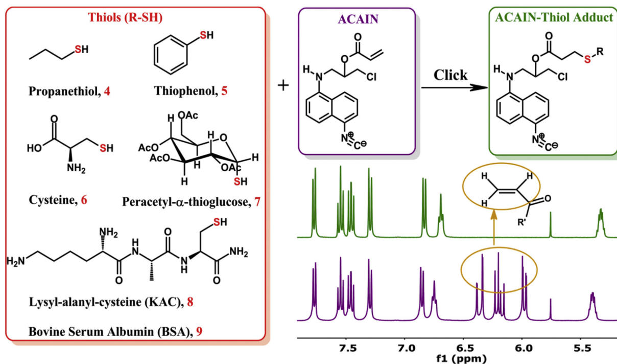
Fig. 2. The thiol-ene click reaction of ACAIN with different thiols. The inset NMR spectra show the aromatic and olefin region of ACAIN (purple, bottom) and the ACAIN-propanethiol reaction mixture after 5 min (green, top). (For interpretation of the references to colour in this figure legend, the reader is referred to the web version of this article.)
