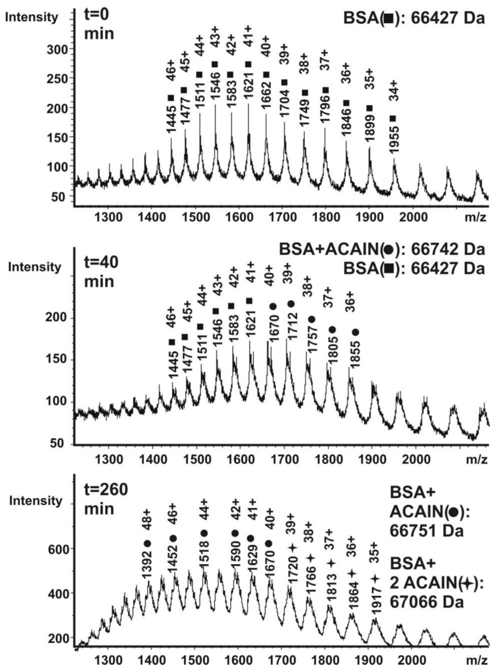
Fig. 6. The mass spectra of the reaction mixture of the BSA and ACAIN at different reaction times. The peaks are marked with the corresponding masses and the charge state of the ions. Experimental conditions: [BSA]_0 = 0.52 mM, [ACAIN]_0 = 1.04 mM in water/DMSO (50/50 V/V) at 25 °C.
