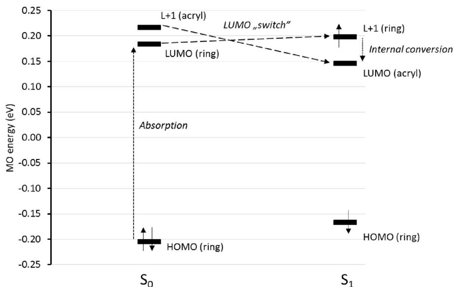
Fig. 8. LUMO “switch” during the relaxation into the S_1 geometry giving rise to an internal conversion into a dark state. The MO energy values are taken from Hartree-Fock single point calculations on the ground and first excited geometries calculated by DFT.
