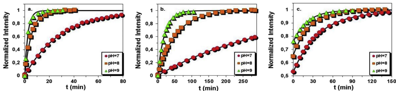
Fig. 4. The fluorescence intensity versus time curves for the reaction of ACAIN with cysteine (a) ( \lambda_{em} = 505 nm), KAC (b) ( \lambda_{em} = 505 nm) and BSA (c) ( \lambda_{em} = 460 nm). Experimental conditions: [cysteine]_0 = [KAC]_0 = [BSA]_0 = 50 \mu M , [ACAIN]_0 = 6.3 \mu M , T = 20^\circ C . The relative intensities are given as (I - I_0)/(I_\infty - I_0) , where I is the intensity at time t , I_0 the initial and I_\infty the final fluorescence intensity.
