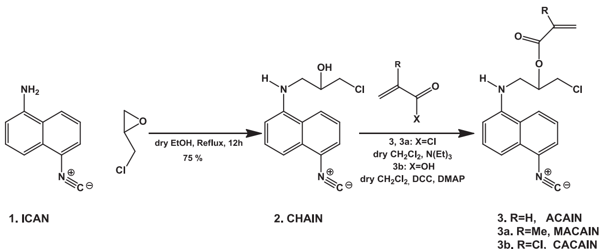
Scheme 1. Synthesis of 1-(3-chloro-2-hydroxyprop-1-yl)-amino-5-isocyanonaphthalene (2, CHAIN), 1-(2-acryloyloxy-3-chloro-prop-1-yl)-amino-5-isocyanonaphthalene (3, ACAIN), 1-N-(2-methacryloyloxy-3-chloroprop-1-yl)-amino-5-isocyanonaphthalene (3a, MACAIN) and (2-chloroacryloyloxy-3-chloroprop-1-yl)-amino-5-isocyanonaphthalene (3b, CACAIN).
