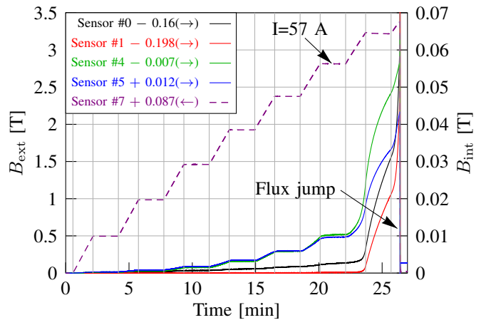
Fig. 5. Color online. Magnetic field measured by the external (dashed lines) and internal (solid lines) Hall sensors, after offset (trapped field) subtraction (see text for details). The vertical lines indicate the start and end of the ramps. Plateaus correspond to integer multiples of 9.5 A magnet current. Ramp rate is 0.1 A/s. Arrows in the legend indicate the vertical axis.
