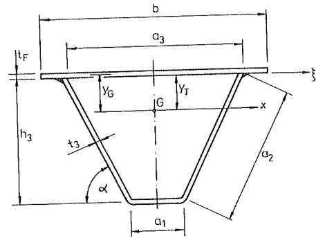
Figure 4. Dimensions of a trapezoidal stiffener
