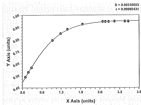
Figure 5. Curvefit for the standard normal probability.
