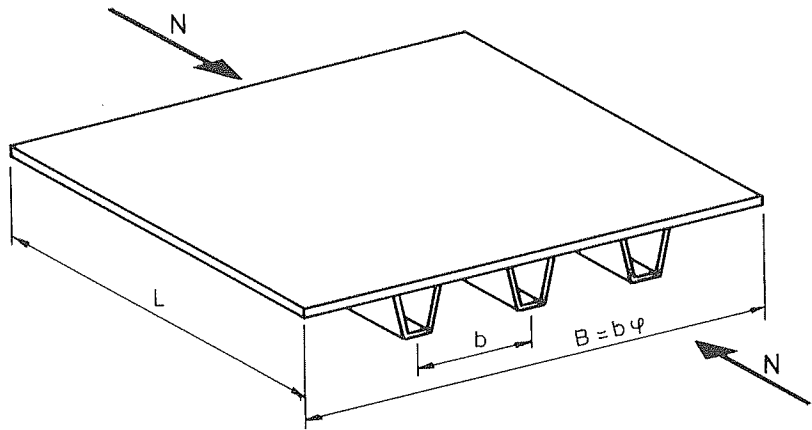
Figure 1. A uniaxially compressed longitudinally stiffened plate
