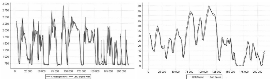
(a) Engine speed (RPM) (b) Vehicle speed Figure 9: Comparing charts in ObdCanCompare report
