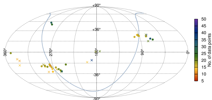
Fig. 10. The distribution in the sky of various Cepheid-type stars from the Gaia DR2 classifications crossmatched with Kepler and K2 measurements. Crosses mark stars we rejected or were not able to confirm: half of these are at high Galactic latitudes. The notation is the same as in Fig. 2.
