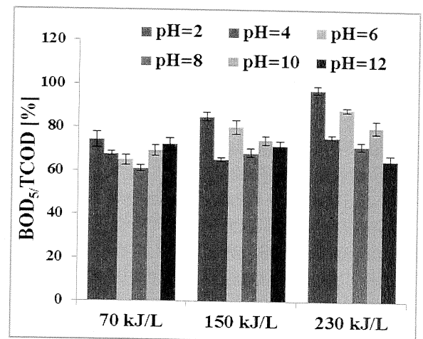
Figure 2. BOD/TCOD for pre-treated sludge
