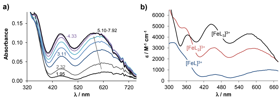
Fig. 3. UV-Vis absorption spectra recorded for the iron(III) – Q-3 (1:3) system at different pH values (a) and calculated UV-Vis molar absorption spectra of the various complexes (b). ( c_{\text{Q-3}} = 50 \mu\text{M} ; T = 25.0 \text{ }^\circ\text{C} ; l = 0.20 \text{ M KCl} ; l = 2 \text{ cm} ).
