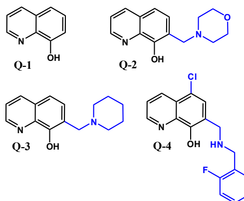
Chart 1. Structures of the reference compound 8-hydroxyquinoline ( Q-1 ) and its derivatives ( Q-2 , Q-3 , Q-4 ) reported in this work in their neutral form.
