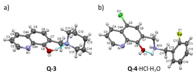
Fig. 1. ORTEP views of Q-3 (a) and Q-4·HCl·H 2 O (b) at 30% probability level of displacement ellipsoids. Blue lines indicate the suggested intramolecular hydrogen bonds. Selected bond distances and bond angles are listed in Tables S2, S4.
