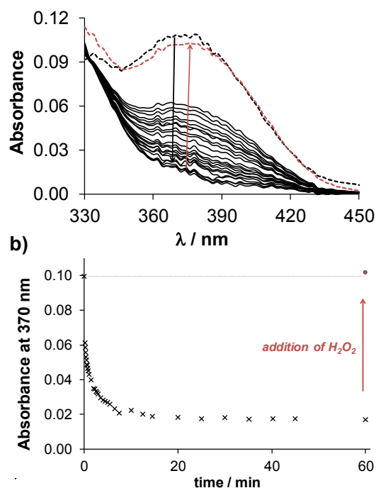
Fig. 8. Time-dependent UV-Vis spectra of the copper(II) complexes of Q-2 (a) upon addition of 2.5 equivalents of GSH at pH 7.40. Black dashed lines denote the initial spectra before addition of GSH, red dashed lines the spectra upon addition of \text{H}_2\text{O}_2 (a). Absorbance values measured at 370 nm plotted against the time (b). ( C_{\text{copper(III)}} = 100 \mu\text{M} ; C_{\text{ligand}} = 100 \mu\text{M} ; C_{\text{GSH}} = 250 \mu\text{M} ; T = 25.0 \text{ }^\circ\text{C} ; I = 0.20 \text{ M KCl} )
