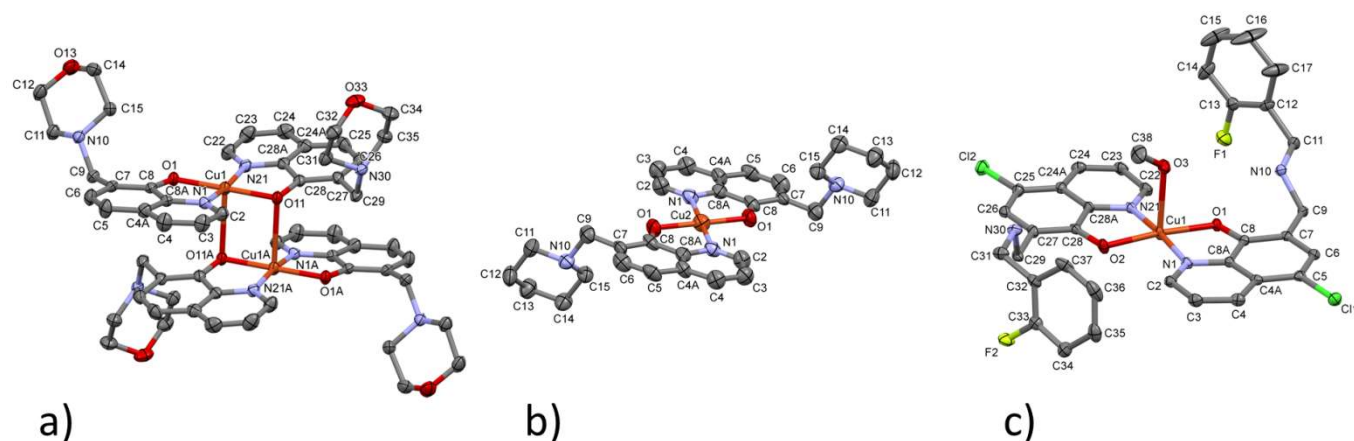
Fig. 5. The cyclic dimer structure of complex cation [(\text{Cu}(\text{HQ-2})_2)_2]^{4+} in [(\text{Cu}(\text{HQ-2})_2)_2] \cdot (\text{CH}_3\text{OH})_2 \cdot \text{Cl}_4 \cdot (\text{H}_2\text{O})_2 (a), [(\text{Cu}(\text{Q-3})_2)]^{2+} in [\text{Cu}(\text{Q-3})_2] \cdot \text{Cl}_2 (b) and [(\text{Cu}(\text{HQ-4})_2(\text{CH}_3\text{OH}))_2]^{2+} in [\text{Cu}(\text{HQ-4})_2(\text{CH}_3\text{OH})] \cdot \text{ZnCl}_4 \cdot \text{CH}_3\text{OH} at 30% probability level of displacement ellipsoids. Hydrogens, as well as the chloride and [\text{ZnCl}_4]^{2-} anions, water and methanol molecules present in the crystal lattice are omitted for clarity. Selected bond lengths (Å) and angles (°) for [(\text{Cu}(\text{HQ-2})_2)_2]^{4+} : Cu1-O1 1.931(3), Cu1-O11 1.954(3), Cu1-N1 1.989(3), Cu1-N21 1.967(3), Cu1-O11A 2.681(3), O1-Cu1-O11 179.5(1), N1-Cu1-N21 171.0(1), O1-Cu1-N1 84.2(1), O1-Cu1-N21 95.7(1), O11A-Cu1-N1 92.8(1), O11A-Cu1-N21 96.1(1), O1-Cu1-O11A 92.4(1), O11-Cu1-O11A 87.2(1). Selected bond lengths (Å) and angles (°) for [(\text{Cu}(\text{Q-3})_2)]^{2+} : Cu2-O1 1.945(6), Cu2-N1 1.951(8), O1-Cu2-N1 85.1(3), O1-Cu2-N1 94.9(3), O1-Cu2-O1 180.0, N1-Cu2-N1 180.0. Selected bond lengths (Å) and angles (°) for [(\text{Cu}(\text{HQ-4})_2(\text{CH}_3\text{OH}))_2]^{2+} : Cu1-O1 1.969(2), Cu1-O2 1.952(3), Cu1-N1 1.989(4), Cu1-N21 1.978(4), Cu1-O3 2.314(4), O1-Cu1-O2 174.53(13), N1-Cu1-N21 174.63(15), O1-Cu1-N1 84.26(11), O1-Cu1-N21 97.11(11), O2-Cu1-N1 93.95(13), O2-Cu1-N21 84.22(13), O1-Cu1-O3 87.43(11), O3-Cu1-N1 97.45(14), O3-Cu1-N21 87.81(14), O1-Cu1-O3 87.43(11).
