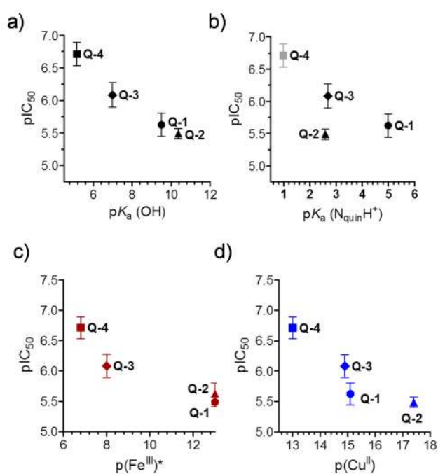
Fig. 6. Correlations between pIC_{50} values measured in MES-SA/Dx5 cell lines ( IC_{50} : mol/L) and pK_a (OH) (a), pK_a ( N_{\text{quinolinidium}}H^+ ) (b), pFe(III)^* (c) and pCu(II) (d) of the studied 8-hydroxyquinolines. Data are taken from Tables 1, 2 and Scheme 2.
