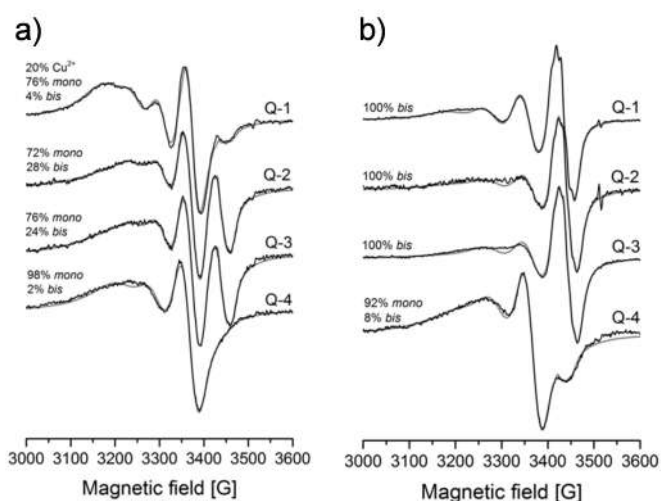
Fig. 4. Experimental (black) and simulated (grey) room temperature EPR spectra recorded for the copper(II) – ligand systems ( Q-1 - Q-4 ) in DMSO at c_{\text{Cu(II)}} = 2 \text{ mM} in the presence of one (a) or two (b) equivalents of the ligand. Concentration ratios of the mono and bis complexes obtained from the simulation are indicated in the spectra.
