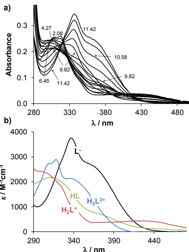
Fig. 2. UV–Vis absorption spectra of Q-2 (a) recorded at different pH values in aqueous solution and the calculated molar absorption spectra of the individual ligand species (b). ( c_{Q-2} = 50 μM; T = 25.0 °C; I = 0.20 M KCl; l = 2 cm)
