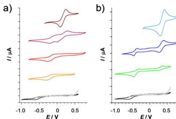
Fig. 7. Cyclic voltammograms of the iron(III) – Q-3 (a) and copper(II) – Q-3 (b) systems. Ligand alone (black / deprotonated: grey), FeCl_3 (brown), iron complexes at the M:L ratios 1:1 (bordeaux), 1:2 (red) and 1:3 (orange), as well as for CuCl_2 (light blue), and copper complexes at the M:L ratios 1:1 (blue) and 1:2 (green). (Potentials measured against Ag/AgCl/KCl (3 M); c_{Q-3} = 1.0 mM; solvent: DMSO; I = 0.01 M (TBAClO 4 ); T = 25 °C; scan rate = 5 mV/s)
