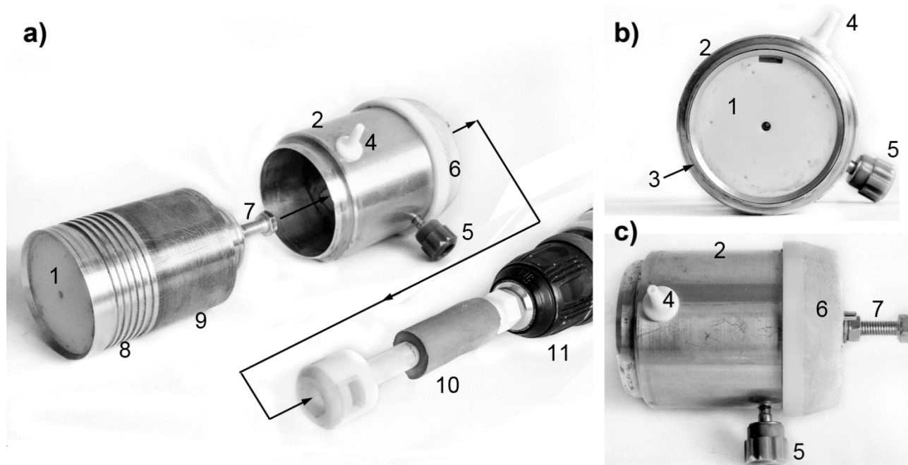
Figure 2. The spinneret in a) exploded, b) top and c) side views. 1: rotor, 2: stator, 3: orifice, 4: solution inlet, 5: high voltage connector, 6: base, 7: hexagonal drive connection, 8: solution take-up thread, 9: sliding bearing, 10: flexible plastic/rubber shaft, 11: chuck
