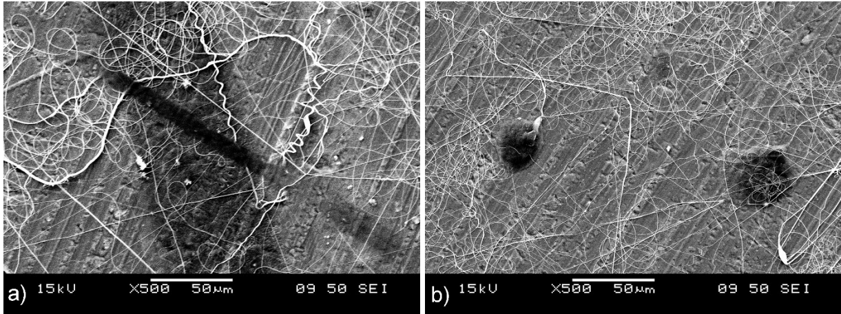
Figure 5. The morphological defects of the samples collected at a) 0 rpm, b) 75 rpm
