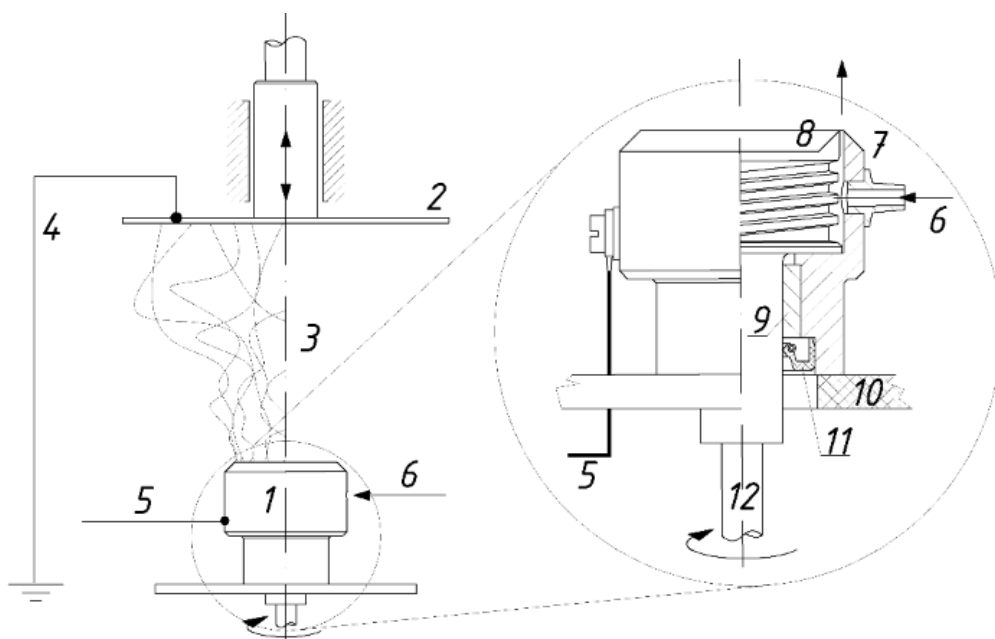
Figure 1. The scheme of the novel electrospinning setup. 1: spinneret, 2: grounded collector, 3: electrospinning space, 4: grounding, 5: high voltage cable, 6: solution feed, 7: stationary part, 8: threaded rotating part, 9: bushing, 10: base platform, 11: lip seal, 12: plastic drive shaft
