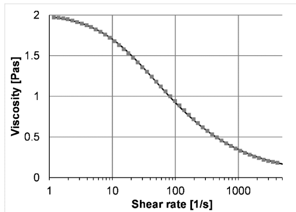
Figure 3. The viscosity of the polymer solution used (dots) and the fitted Cross-Williamson model (continuous line).
