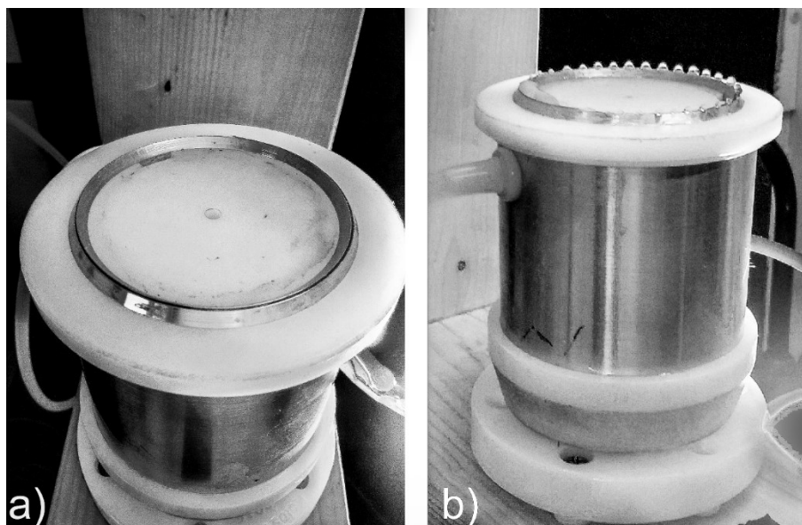
Figure 4. The spinneret mounted to a wooden stand, a) the sharp edges and the annular orifice, b) Taylor-cone formation at 0 rpm
