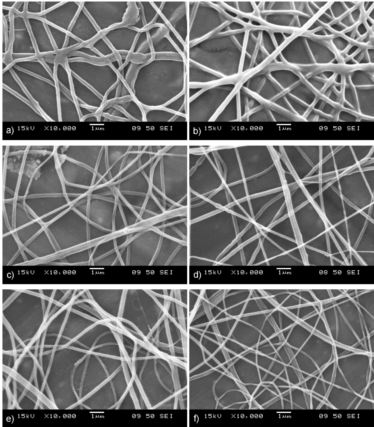
Figure 6. Fibers collected at different rotation speeds, a) 0 rpm, b) 75 rpm, c) 150 rpm, d) 300 rpm, e) 500 rpm, f)750 rpm
