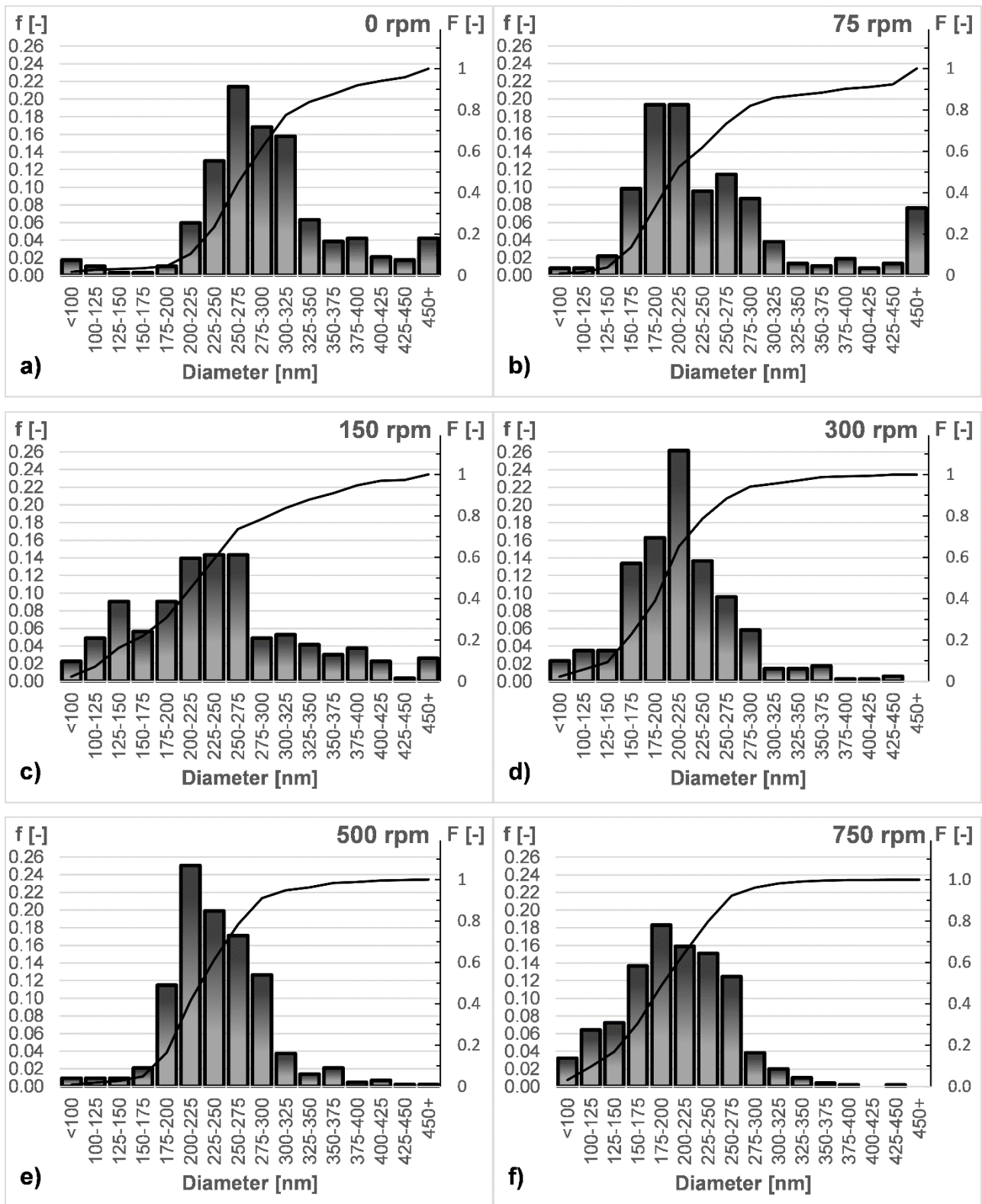
Figure 7. Fiber diameter histograms of the nanofibers electrospun at different rotational speeds
