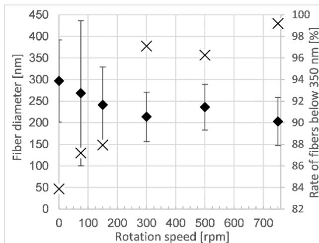
Figure 8. Average fiber diameters with standard deviation (♦) and the rate of faultless fibers with less than 350 nm diameter (X) as a function of rotation speed
