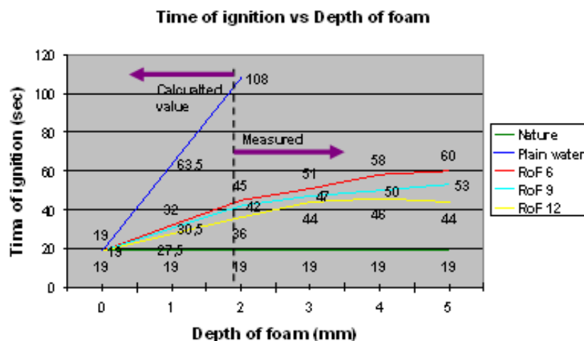
Figure 2 - Measured and interpolated value of ignition time
