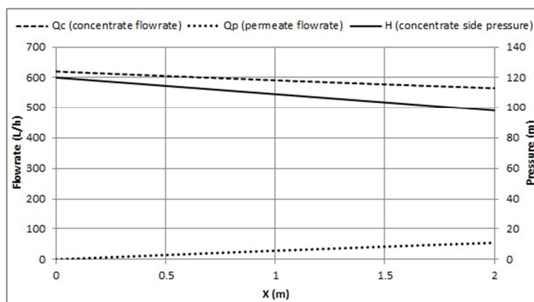
Fig. 4. Calculated head-loss and flow-rate profile at higher dissolved iron concentrations
